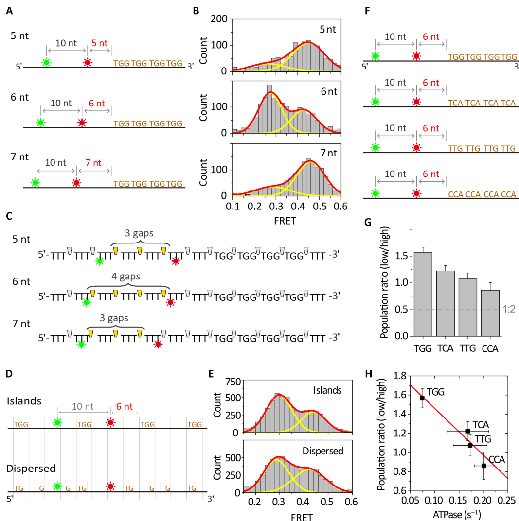
Fig. 3. Phase bias due to 3-nt-period sequence pattern. (A) DNA designs with different distances (5, 6, and 7 nt) between TGG repeats and a dye pair. The interdyne separation was kept at 10 nt. (B) The population distributions obtained from the 5-, 6-, and 7-nt dye-to-TGG separations. The population ratios (low to high FRET state) determined by Gaussian fitting of each peak are 1:3.3, 1.5:1, and 1:3.3 for 5-, 6-, and 7-nt dye-to-TGG distances, respectively. (C) Schematic of the base grouping and gap generation in which the bases are grouped into "TGG" that account for the data in (B). Each DNA shows a different number of the gaps between the two dyes depending on their dye-to-TGG distance. (D) DNA designs with different base distributions. In the sequence named "islands," the four triplets of TGG were distributed along the DNA, whereas their positions from the dye pairs are kept in phase. In the sequence "dispersed," the guanine bases were displaced further, whereas their positions are kept in phase. (E) The population distributions obtained from the islands and dispersed. The population ratios (low to high FRET state) determined by Gaussian fitting of each peak are 1.8 and 1.6 with islands and dispersed, respectively. (F) DNA designs with different triplet sequences placed 6 nt apart from the dye pair of a 10-nt separation. (G) The population ratio (low FRET to high FRET) observed from the four triplet sequences in (F). Dashed line indicates the 1:2 ratio limit expected from the random distribution. (H) Correlation plot between the population ratios in (G) and the ATP hydrolysis rates measured from the filament formed on the triplet repeats. The ATP hydrolysis rates were adapted from the study of Kim et al. (38). All the measurements were carried out in the presence of 1 mM ATP.
