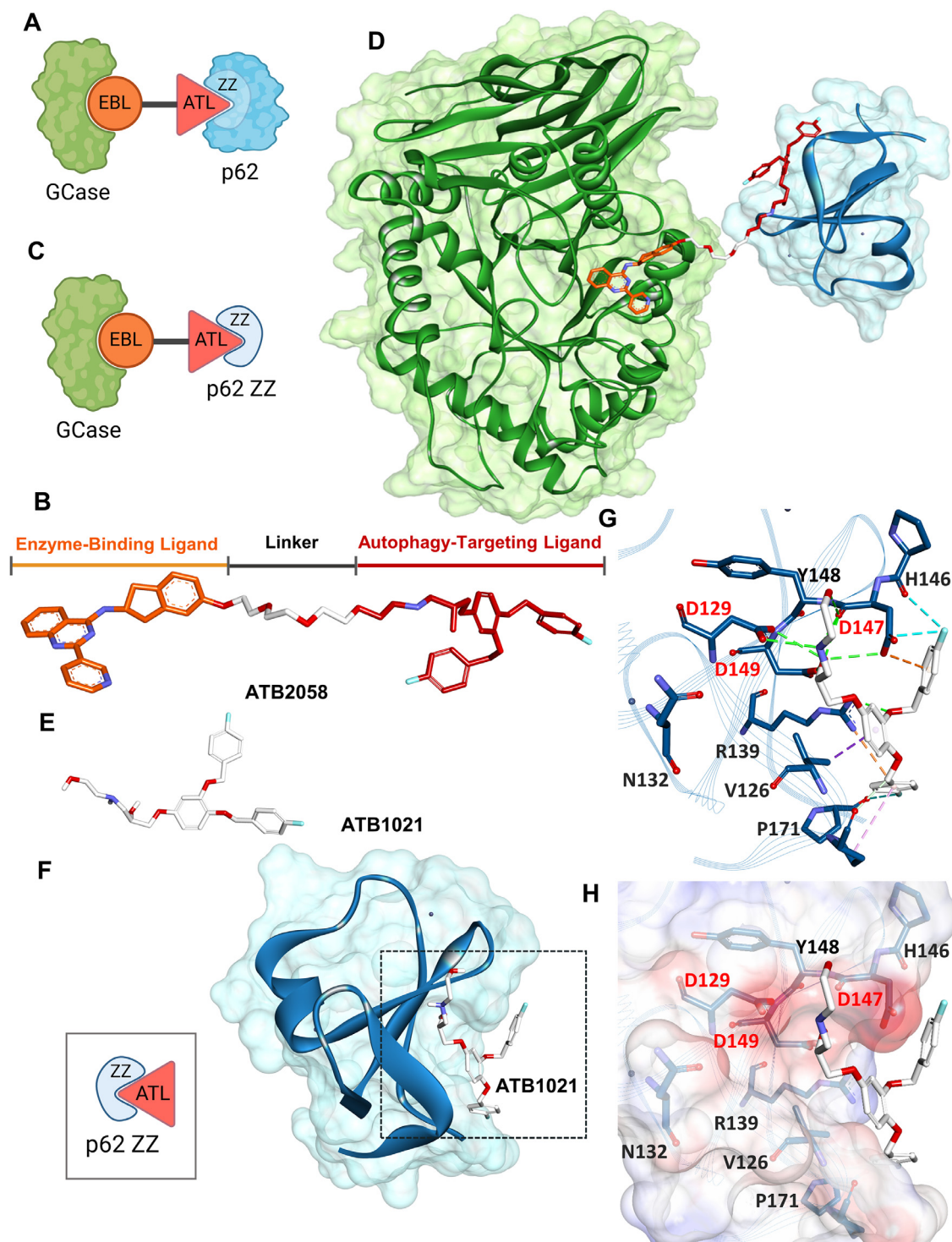
Fig. 2 – Structural analysis of the LYSOTAC compound binding to GCase and p62 ZZ domain. (A) Design of a LYSOTAC compound binding to both GCase and p62 ZZ domain; (B) 3D structure of ATB2058 shown as a stick model, consisting of EBL (orange), linker (white), and ATL (red); GCase is shown in green and the p62 ZZ domain in blue, displayed in both cartoon (C) and semi-transparent surface representations (D). The LYSOTAC molecule is visualized in the same stick model and color scheme as illustrated in (B); (E) 3D structure of the ATL depicted as a white stick model; (F) Representative binding conformation of the ATL and p62 ZZ domain (blue) displayed in both cartoon (left panel) and semi-transparent surface representations (right panel); (G, H) Interaction analysis of ATB1021 with p62 ZZ domain, with the electrostatic surface. Hydrogen bonds, alkyl, \pi -alkyl, halogen bonds and electrostatic interactions are represented by dashed lines in green, pink, purple, cyan and orange, respectively. Key interacting residues are colored in red. Cartoons were created in BioRender. Park, J. (2026) https://BioRender.com/6qf7ykt .
