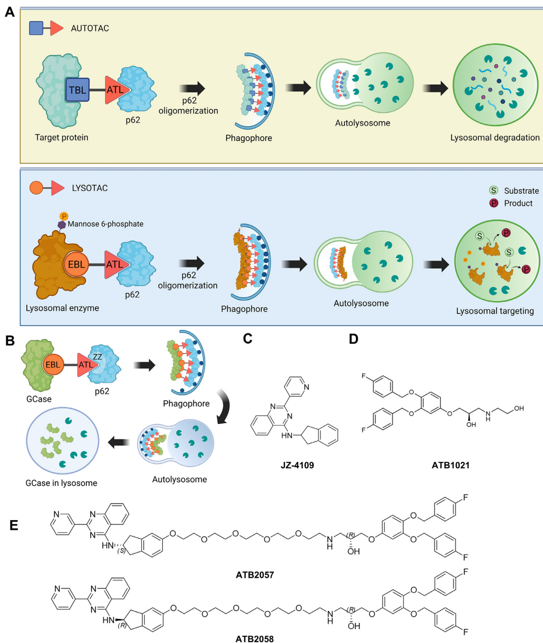
Fig. 1 – Development of LYSOTAC compounds. (A) Schematic diagram of LYSOTAC technology compared to AUTOTAC (Created in BioRender. Park, J. (2026) https://BioRender.com/ijm1ere ); (B) Schematic diagram of a LYSOTAC compound designed to deliver GCase to lysosomes (Created in BioRender. Park, J. (2026) https://BioRender.com/nxs6jn7 ); (C-D) Chemical structures of JZ-4109 used as EBL, ATB1021 used as ATL, and ATB2057 and ATB2058 generated as LYSOTAC compounds targeting GCase.
