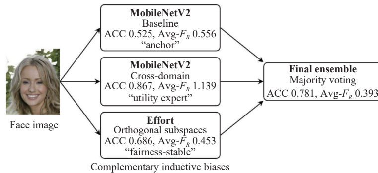
Fig. 9 Team ICI Innolabs: Architecture combining complementary inductive biases via majority voting
