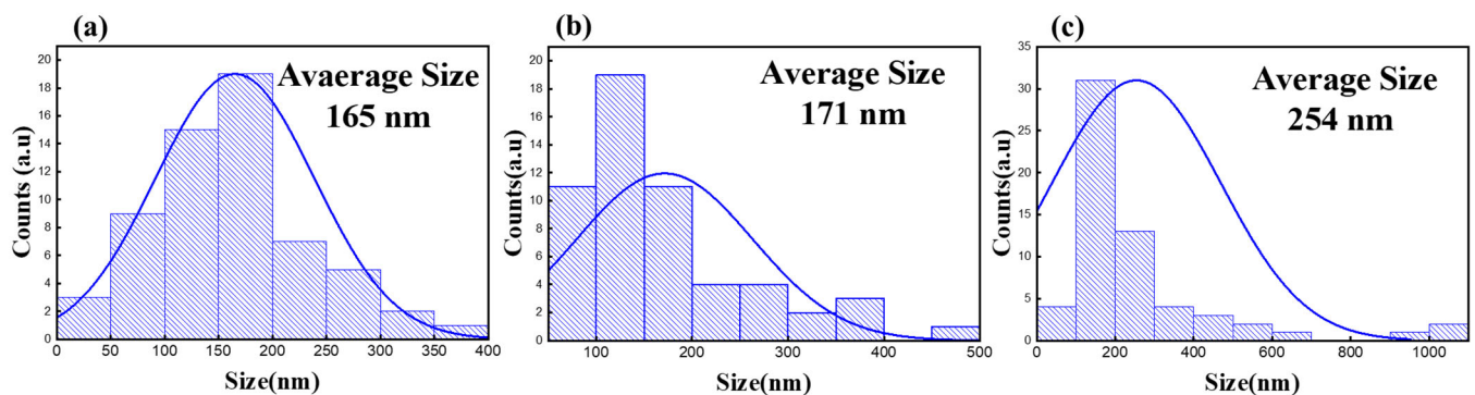
Figure 5. Variation in the hole diameter of the cottonwood pollen surface based on current application time, (a) no current, (b) 1 mA for 1 s, (c) 1 mA for 2 s.
