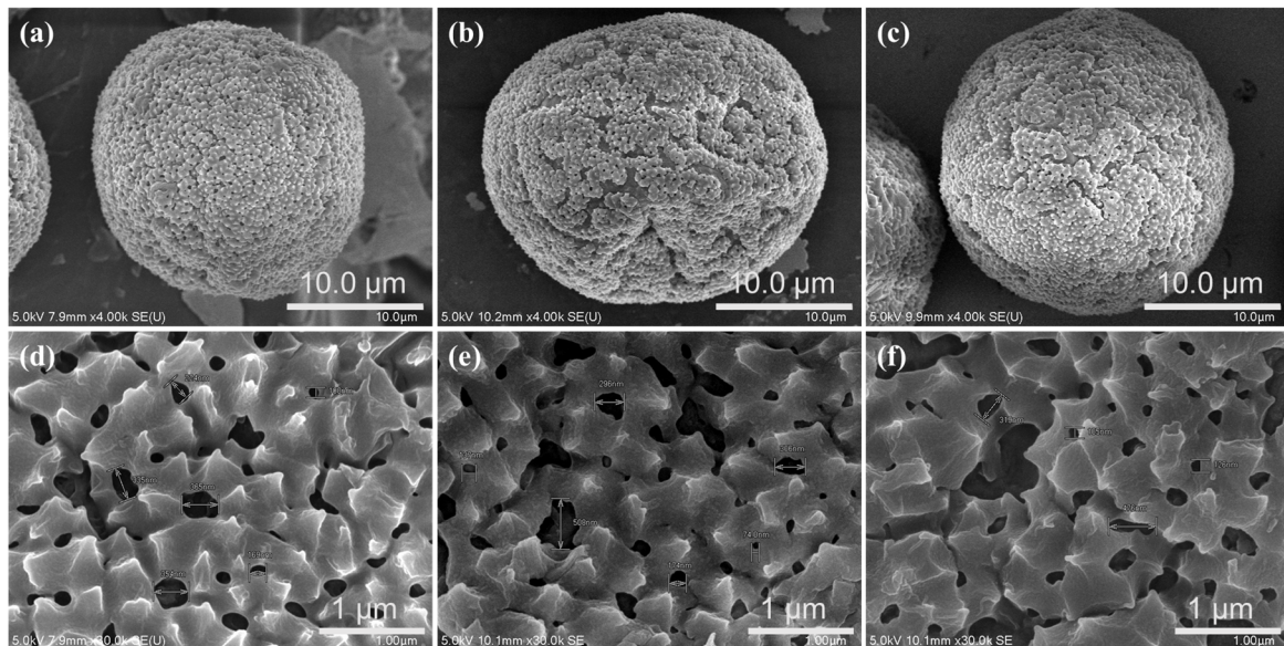
Figure 4. Variation in pollen surface on PP + Ag filter according to current application time: (a,d) before current application, (b,e) 1 s and (c,f) 2 s after application.
