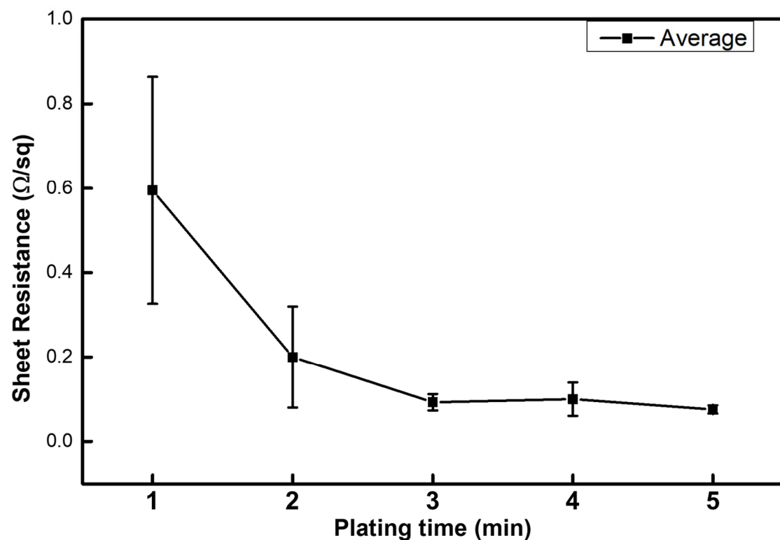
Figure 3. Sheet resistance change in PP + Ag filter according to the Ag electroless plating time.
