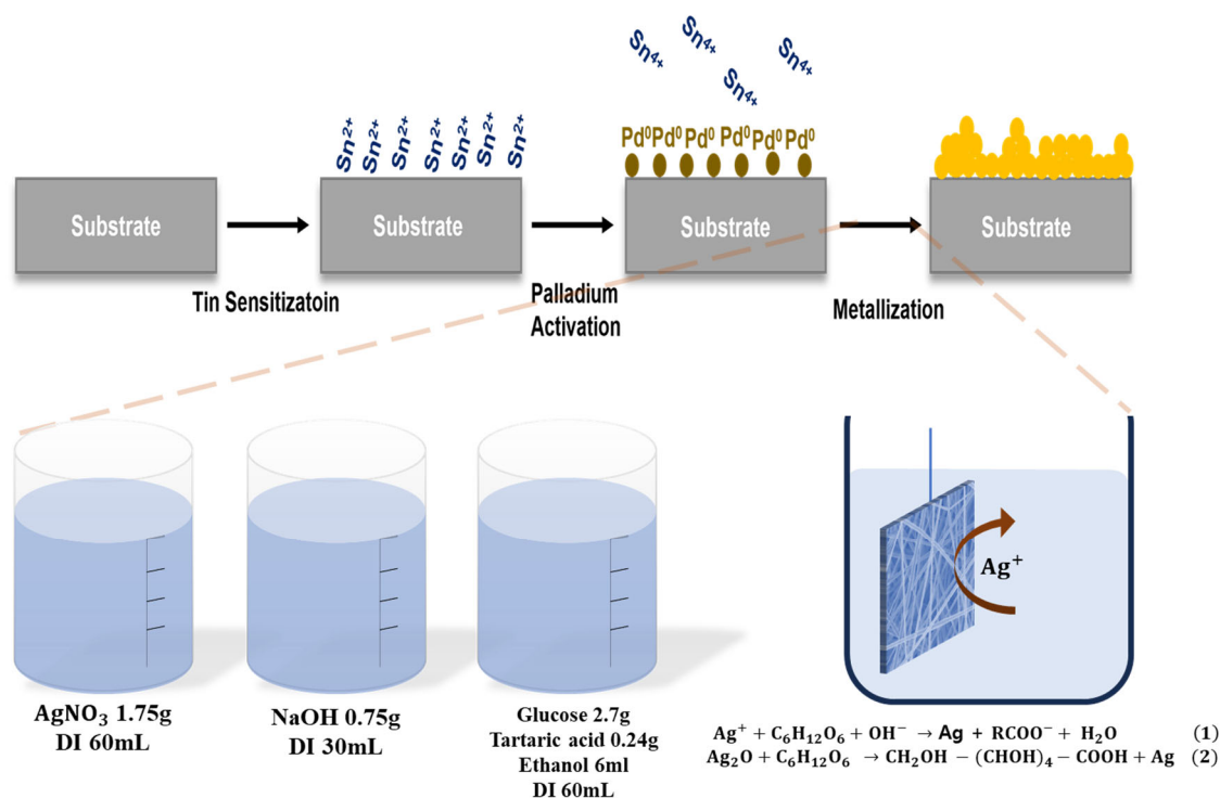
Figure 1. Experimental procedure for the electroless Ag plating process.
