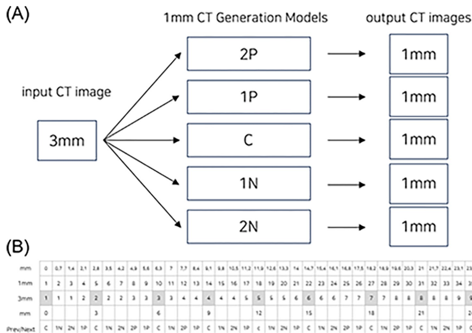
Fig 5. Configuration of 3 mm CT image input and multiple 1 mm generative models (A) and the example of slice location mapping table (B). The grey column within the 3 mm image means the matched area on the 1 mm image. The 1 mm image corresponding to 3 mm was used in the Typo, and 1 mm images adjacent to 3 mm were used for training the 2P, 1P, 1N, and 2N models, respectively. C, corresponding; 2P, before 2 slices; 1P, before 1 slice; 1N, after 1 slice; 2N, after 2 slices.
