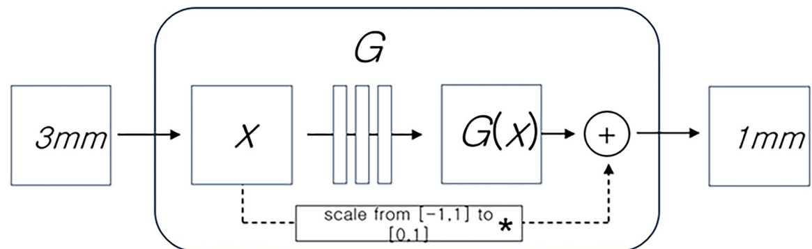
Fig 6. Two models for generating 1 mm slice CT images from 3 mm images: (A) Method 1, (B) Method 2. (A) 'Method 1' used a 3 mm CT raw image ( x ) as the input image and was configured to generate a 1 mm CT raw image ( G(x) ). (B) 'Method 2' used 3 mm CT raw image ( x ) as the input image, and the difference values between 3 mm and 1 mm CT images ( * ) were trained. The different value was added to create 1 mm CT images ( + ). X , CT 3 mm input image; G , generative model; G(x) , generated results.
