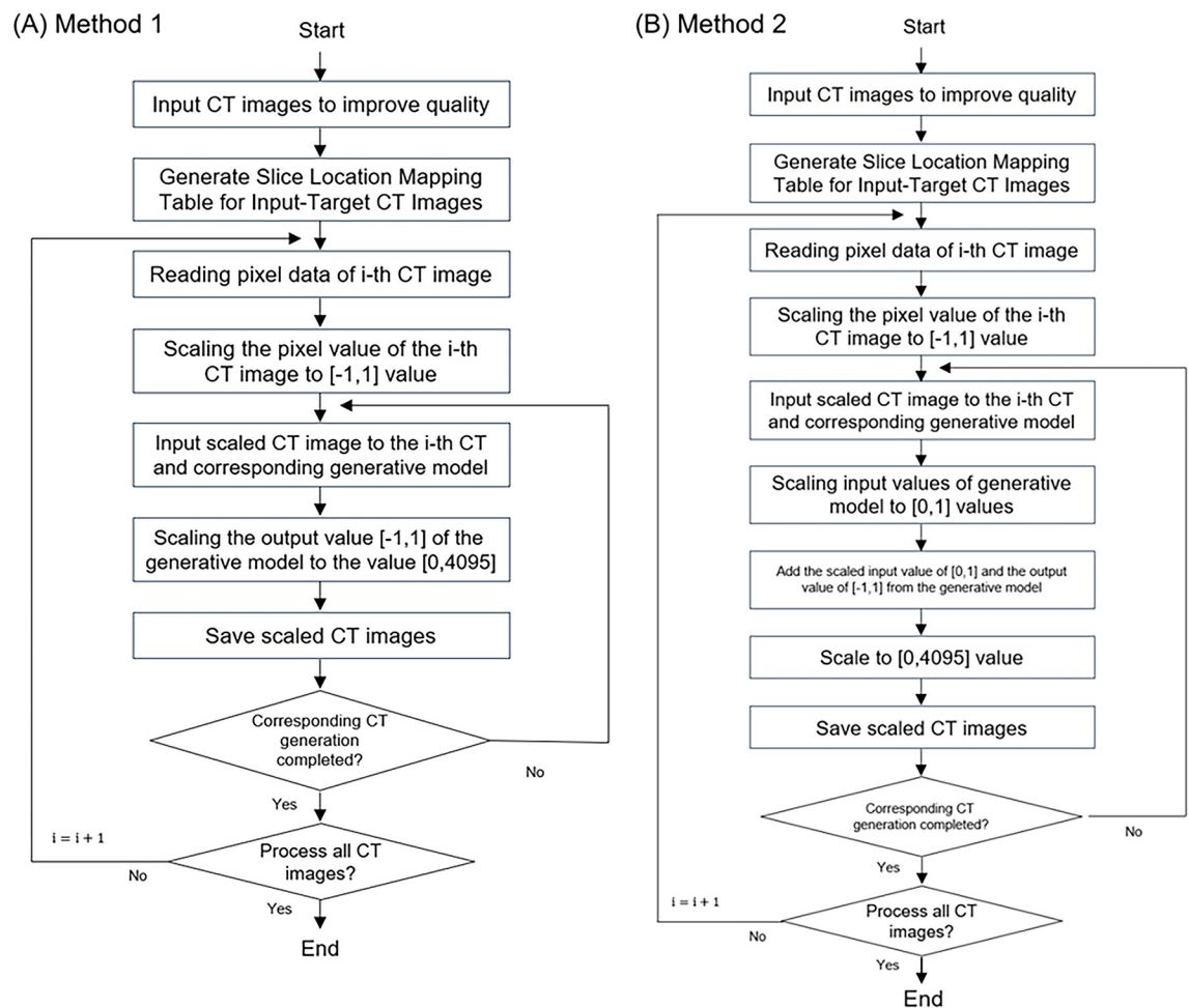
Fig 3. Flow chart. This flow chart illustrates the process of converting N sheets of 3 mm CT images into their corresponding 1 mm counterparts using two methods within a cGAN model. Each 3 mm CT image is processed individually and the operation is repeated N times. In Method 1 (A), the i -th 3 mm CT image's pixel value is read and input into the cGAN model in the range of [-1,1] . The model then generates an output that is scaled from the range [-1,1] to fit the CT image pixel value range of [0,4095] . Method 2 (B) also starts by reading the i -th 3 mm CT image's pixel value and inputting it into the cGAN model in the range of [-1,1] . However, this method involves an additional step where the scaled input value [0,1] is added to the output value [-1,1] of the generation model. The final step in both methods involves determining whether the 1 mm slices at positions 2P, 1P, C, 1N, and 2N, relative to the original 3 mm slice, have been created successfully. The generated 1 mm CT image is saved, and the process concludes when there are no more 3 mm CT images to be processed.
