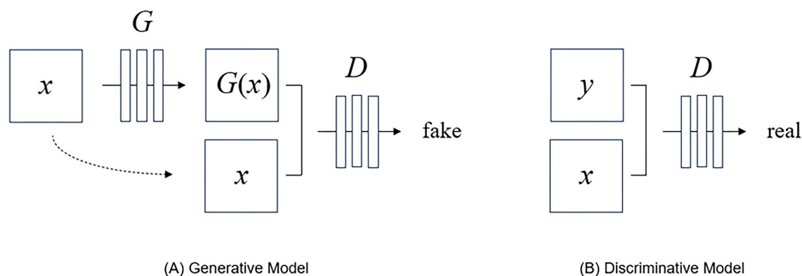
Fig 2. Conditional GANs model. (A) It represents a generative model that generates a fake image from an input image ( x ). ' x ' is the CT 3 mm input image. (B) It was a discriminative model that distinguishes the generated image into real and fake. ' y ' is the 1 mm correct image. G, generative model; D, discriminative model; G(x) , generated 1 mm CT image.
