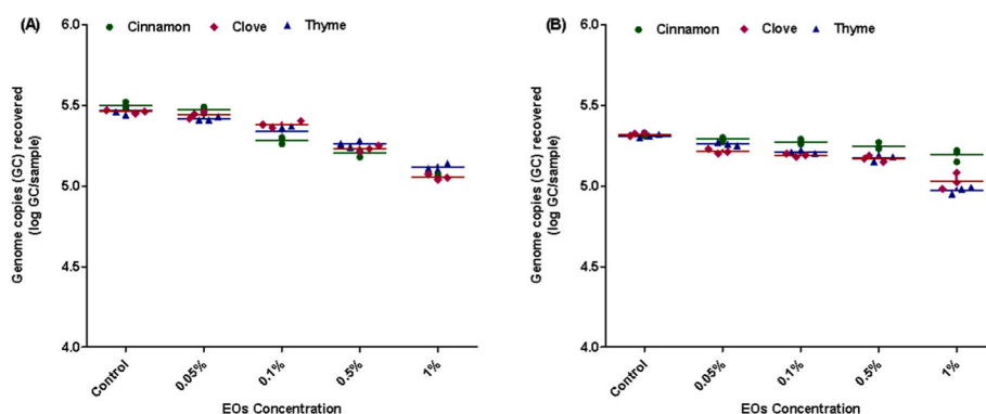
Fig. 5. Effect of EOs (cinnamon, clove, and thyme) on the genomic copy changes of HAV on (A) SS and (B) Kraft paper detected via RT-qPCR.
