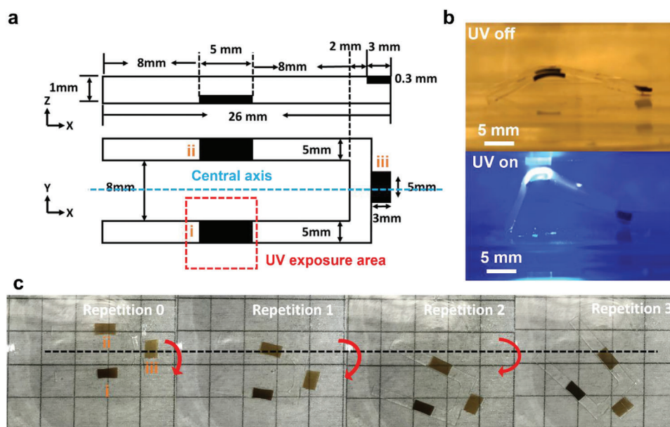
Figure 7. Biomimetic soft steering actuator. a) design of soft steering actuator with three hinges (i, ii, and iii) and selective actuating hinge (i) by UV exposure at 1.1 \text{ W cm}^{-2} ; b) optical images of the side view of steering actuator when UV source was turned on and off; c) the steering process of the soft actuator under interval UV light on a grid background. Each grid has a length of 10 mm. The red dotted lines in (a) were used to indicate the contour of the hinge-based bilayer structure. The black dotted line in (c) indicates the original position of geometric symmetry through repetition 0 to 3.
