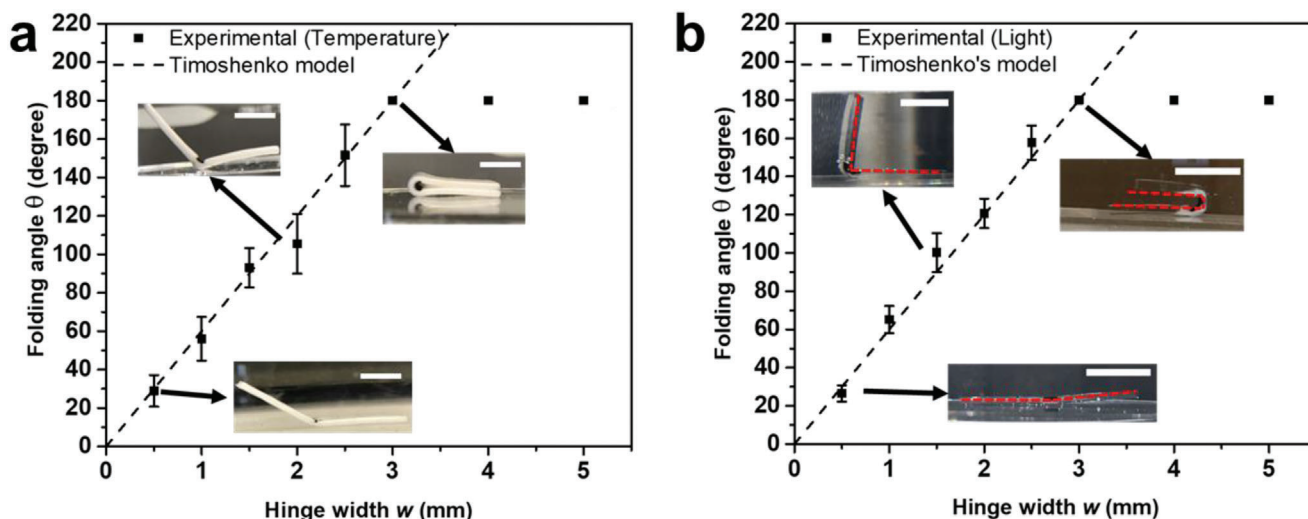
Figure 3. Sample deforms to a folding angle \theta due to anisotropic deswelling between the GO-PNIPAM hinge and the PNIPAM matrix in response to a) temperature and b) light actuation. Measured (dots) and predicted (dash line) \theta are as a function of the hinge width. The predicted result corresponds to the modified Timoshenko's bimorph model. The error bars capture the first standard deviation with a minimum of five samples of each hinge width with all other variables held in constant. Inserted images are folded samples with different hinge widths. The red dotted lines in the inset images were used to indicate the contour of the bilayer structure. Scale bar is 5 mm.
