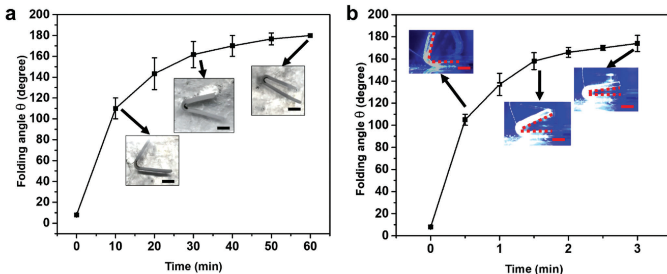
Figure 4. Kinetics of bilayer structure by a) temperature and b) light actuation. The hinge size is 5, 5, and 0.3 mm in width, length, and thickness, respectively. Matrix size is 25, 5, and 1 mm in width, length, and thickness, respectively. Both sizes are measured at the as-prepared state. For temperature actuation, the hydrogel was immersed in water at 38 °C. For light actuation, 1.1 W cm -2 365 nm UV was used. Scale bar is 5 mm.
