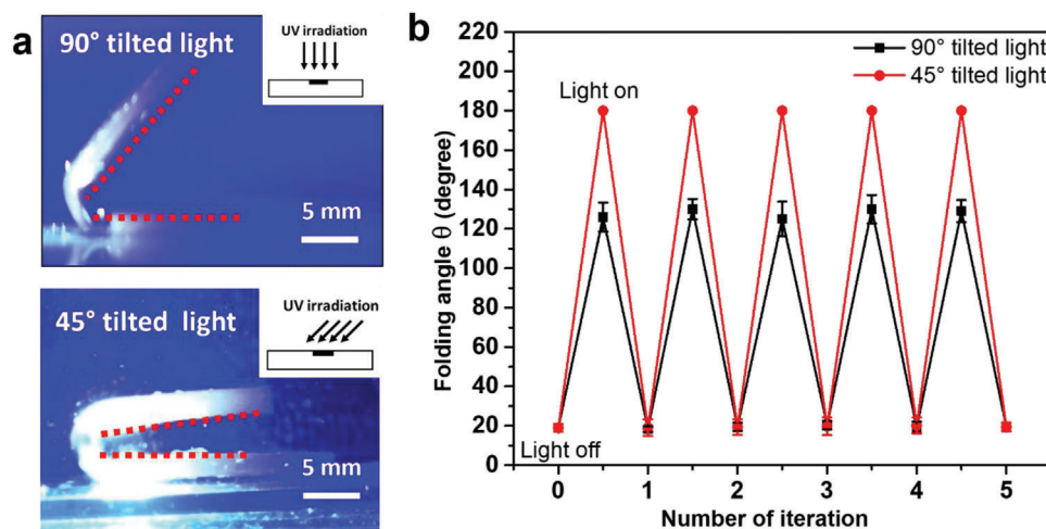
Figure 5. a) Bilayer structures folded after exposure of 90° and 45° tilted light. b) Reversibility of folded bilayer structure by different light directions. The hinge width was 5 mm. The intensity of UV light was kept as 1.1 \text{ W cm}^{-2} throughout the entire experiment. The red dotted lines were used to indicate the contour of the bilayer structure. The inserted images are schematics of light direction.
