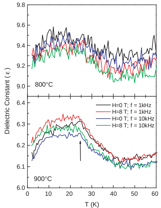
Fig. 4. Temperature dependent dielectric constant \epsilon , in different frequency range, with an applied magnetic field of 0 and 8 T. The applied electric field direction is perpendicular to the external magnetic field.
