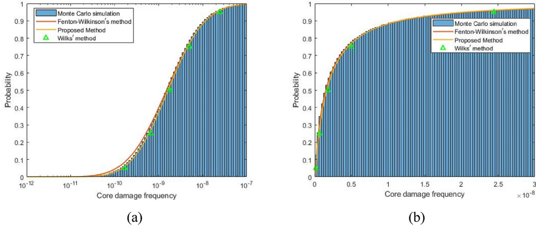
Fig. 2. Cumulative distribution functions for benchmark using Monte Carlo simulations, Fenton-Wilkinson's method, Wilks's method, and the proposed method in the (a) log scale and (b) linear scale.
