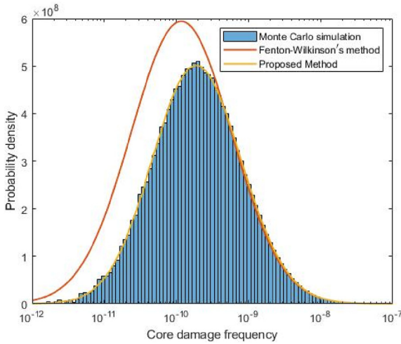
Fig. 3. Probability density functions for the example with Monte Carlo simulations, Fenton-Wilkinson's method, and the proposed method.
