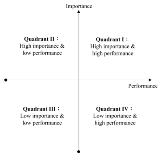
Fig. 3. Importance-Performance Matrix
