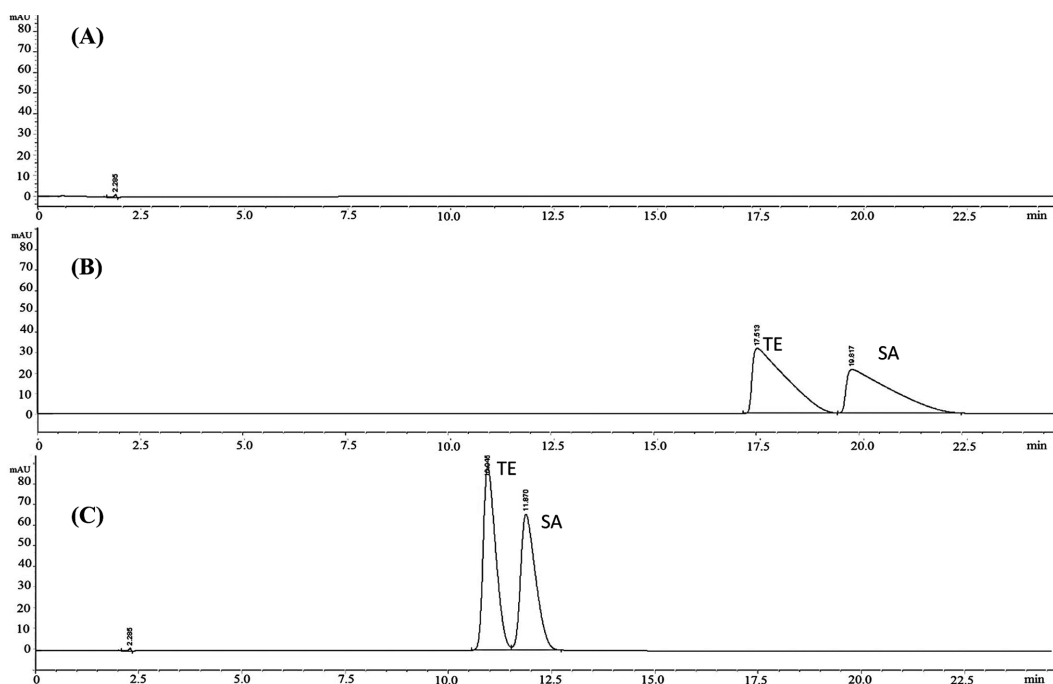
Fig. 2. Typical chromatograms of blank (A); standard mixtures eluted with mobile phase without the addition of RTIL (B) and with [EMIM][Br] (C). Condition: Aegispak C8 column ( 150 \times 4.6 \text{ mm} , 5.0 \mu\text{m} ) 28^\circ\text{C} . Mobile phase consisted of 10 mmol/L potassium dihydrogen phosphate (pH 3.0 adjusted with phosphoric acid) and 40 mmol/L [EMIM][Br]. Flow rate was 1.0 mL/min, injection volume was 10 \mu\text{L} , and detection was at 276 nm. TE: Terbutaline; SA: Salbutamol.
