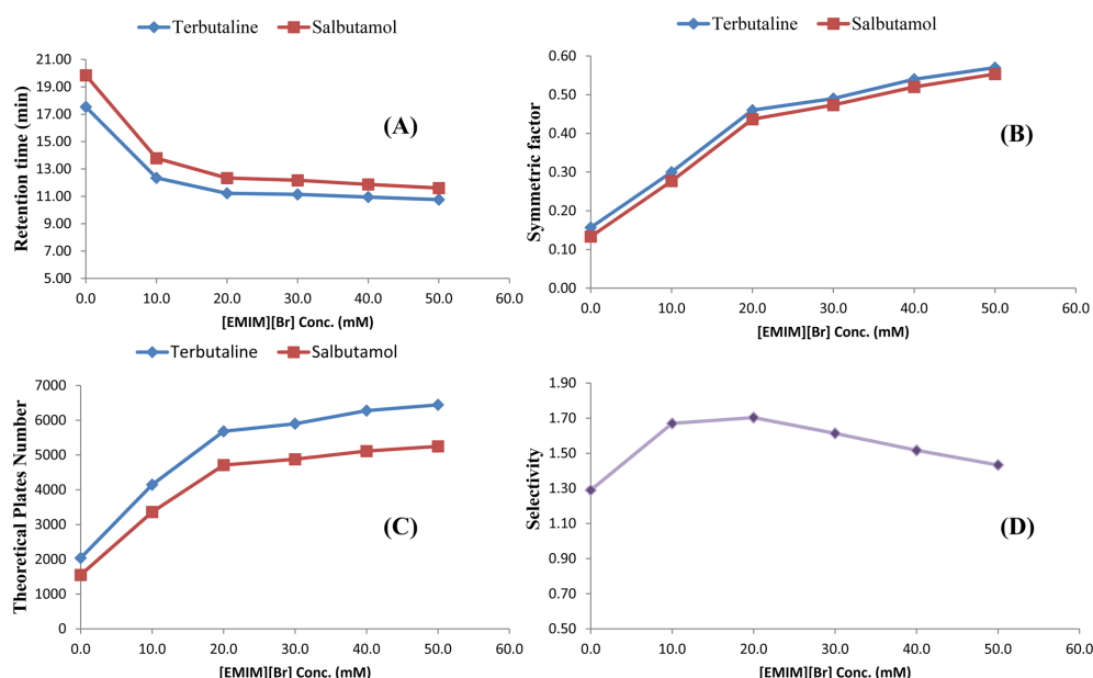
Fig. 4. Effects of [EMIM][Br] concentration on chromatographic behaviors of analytes.
