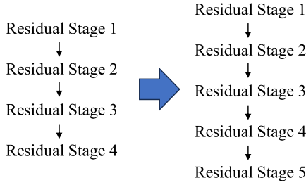
FIGURE 4. DNN architectural changes from the baseline [11] to the proposed model. a) First, a max-pooling layer is added to the stem stage of the baseline. b) Then, an additional residual stage is attached. c) Basic blocks of the baseline are replaced with bottleneck blocks. When s = 2 , average-pooling is performed instead of strided convolution. d) Finally, two 3 \times 3 \times 3 convolutions are added to the stem stage.
