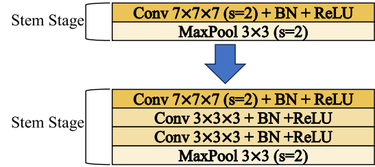
FIGURE 4. DNN architectural changes from the baseline [11] to the proposed model. a) First, a max-pooling layer is added to the stem stage of the baseline. b) Then, an additional residual stage is attached. c) Basic blocks of the baseline are replaced with bottleneck blocks. When s = 2 , average-pooling is performed instead of strided convolution. d) Finally, two 3 \times 3 \times 3 convolutions are added to the stem stage.
