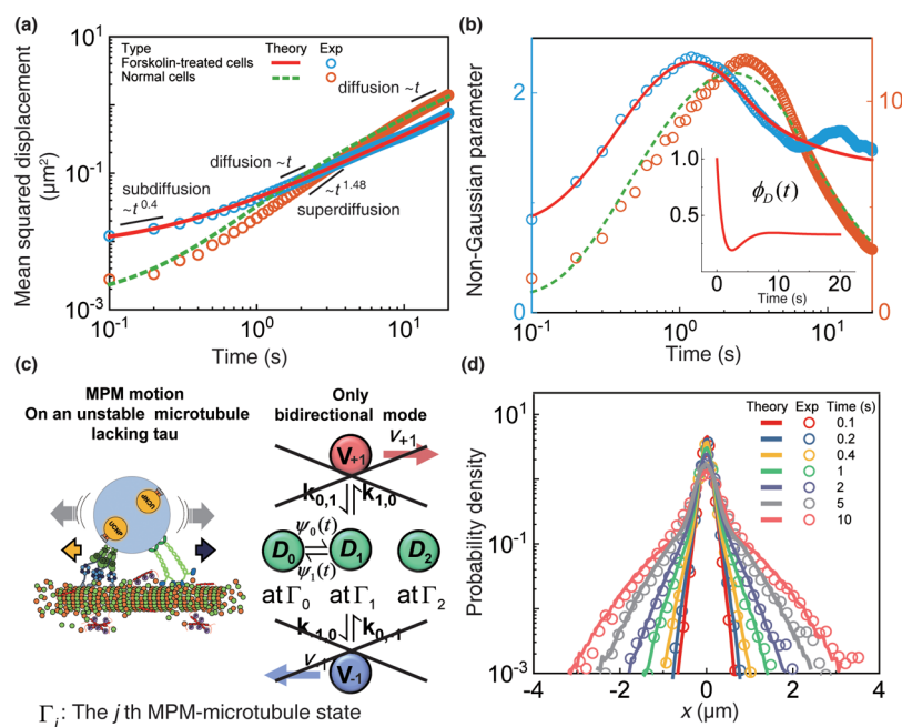
Figure 2. Mean square displacement, non-Gaussian parameter, and distribution of the vesicle motor protein multiplex's displacement along the microtubule. (a and b) Mean square displacement (MSD) and non-Gaussian parameter (NGP) of VMPM motion along the microtubule: (blue circles) experiment results of the forskolin-treated cells, (red line) theoretical result of eqs 1a and 1b (see also Materials and Methods ), (orange circles) experiment results of the normal cells, and (green dashed line) theoretical result of the multimode MPM model (see Supplementary Method 2 in ref 17). In forskolin-treated cells, the MSD time-profile of VMPMs exhibits the direct transition from the initial subdiffusion to ultimate diffusion without transient superdiffusion that emerges in the MSD time-profile in normal cells; at short times, liberational motion of a vesicle bound to the MPM makes the dominant contribution to the MSD of the VMPM and at long times, diffusive motion of the MPM makes the dominant contribution to the MSD, i.e., \langle d_x^2 \rangle \cong 2\langle D_T \rangle t . (inset of B), The normalized time correlation function, \phi_D(t) \equiv \langle \delta D_T(t) \delta D_T(0) \rangle / \langle \delta D_T^2 \rangle , of diffusion coefficient fluctuation of the MPM, extracted from the MSD and NGP data using eq 2 without assuming a particular model. Using the time-profile of \phi_D(t) , we construct the explicit model of the MPM motility fluctuation, shown in (c). In (b), the left-y axis and right y-axis represent the NGP value in the forskolin-treated cells and the NGP value in the normal cells, respectively. (c) Schematic representation of the MPM motion on an unstable microtubule lacking tau in the forskolin-treated cells. Unidirectional motion of the MPM is suppressed. MPMs only bidirectional random motion with a partially dynamic motility fluctuation. Our model of the MPM motion with motility fluctuation is schematically represented. D_i designates the effective diffusion coefficient of the MPM in state \Gamma_i . A unified, quantitative explanation of our experimental results for the MSD and NGP time-profile is achieved when the waiting time distribution, \psi_i(t) i \in \{0,1\} of State \Gamma_0 or State \Gamma_1 , is modeled by a gamma distribution (see Materials and Methods ). (d) VMPM displacement distribution in forskolin-treated cells: (circles) experiment results and (lines) theoretical predictions by our model optimized against the MSD and NGP data of VMPM motion in forskolin-treated cells.
