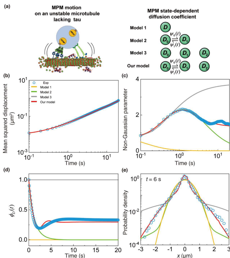
Figure 3. MPM motility fluctuation dependent NGP time-profiles and displace distribution of VMPMs. (a) Various models of the MPM state dynamics. At the MPM state \Gamma_i , the MPM undergoes diffusive random motion with the MPM state-dependent diffusion coefficient, D_i . \psi_i(t) denotes the lifetime distribution of the MPM state \Gamma_i , modeled as a gamma distribution. See Table 2 for the parameter values used in the theoretical calculation for Models 1–3. For our model, the parameter values are listed in Table 1. (b and c) Time-profiles of the MSD and NGP of the VMPM. Theoretical results are calculated by eqs 1a and 1b for all models. (d) Time correlation function of the diffusion coefficient fluctuation calculated for each model. For model 1, \delta D = \phi_D(t) = 0 . For Model 2, the TCF is given by eq 4 with p_2 = 0 . The values of other parameters are given in Table 2. For Model 3, \phi_D(t) = 1 because \langle \delta D_{\Gamma}(t) \delta D_{\Gamma}(0) \rangle = \langle \delta D_{\Gamma}^2 \rangle at all time t . The TCF of Model 3 is given by eq 4 with G(\Gamma_i, t | \Gamma_j) = \delta_{ij} with \delta_{ij} denoting the Kronecker delta. The TCF of our model is given by eq 4. (e) The VMPM displacement distribution (VDD) at 6.0 s. Theoretical results are calculated by numerical inversion of eq 16, 95 where the expressions of \hat{P}(k, s) are given in Table 3 for Models 1, 2, and 3. For our model, \hat{P}(k, s) is given in eq 14. For all models, \tilde{f}(k) in eq 16 is given by eq 13. Models 1, 2, and 3 cannot explain our experimental results of the non-Gaussian parameter and the VDD regardless of the parameter values.
