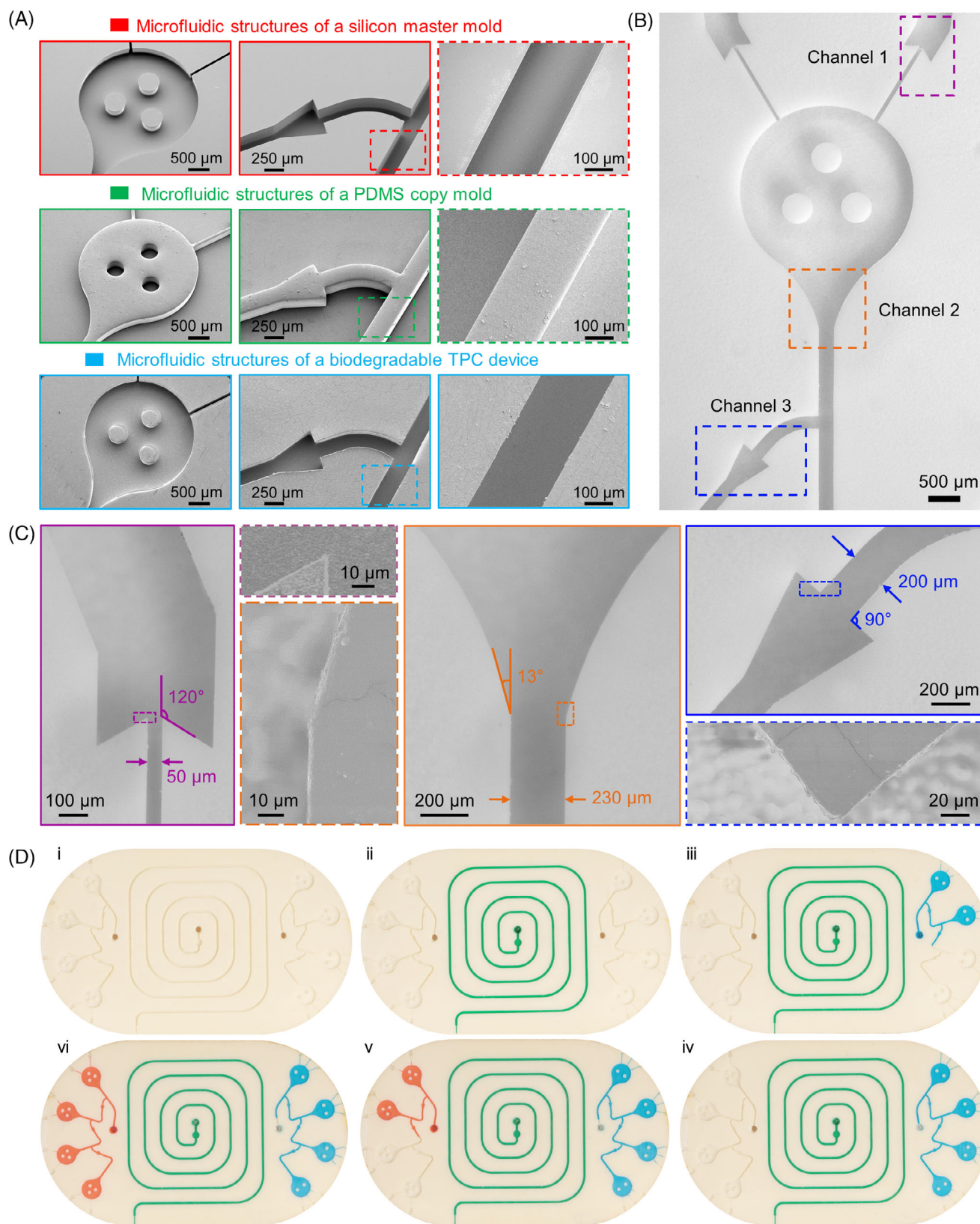
FIGURE 4 Microfluidic structure design and demonstrations of filling guided by capillary bursting valves (CBVs) for chrono-sampling in sequences of reservoirs. (A) Scanning electron micrographs of microfluidic structures on a silicon master mold, a PDMS replica mold, and a layer of TPC. (B, C) Optical images and scanning electron micrographs of three CBVs with indicated channel widths and diverging angles. (D) Optical images demonstrating the working principle of CBVs for chrono-sampling by sequentially filling the channels using dyed artificial sweat. (i) empty device; (ii) filling of the middle microchannel with green dyed artificial sweat; (iii, iv) filling of the microreservoirs on the right with blue dyed artificial sweat guided by capillary bursting valves; (v, vi) filling of the microreservoirs on the left with orange dyed artificial sweat guided by capillary bursting valves
