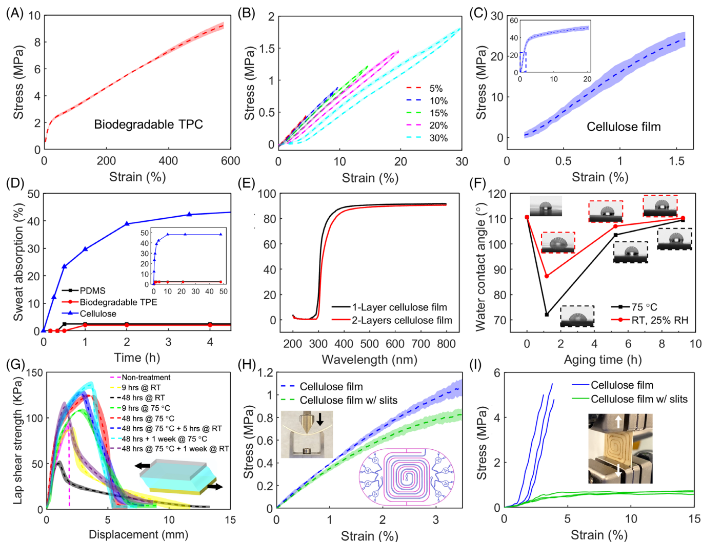
FIGURE 3 Characterization of biodegradable microfluidic systems constructed with TPC and cellulose. (A) The stress–strain behaviors of a sample of TPC during tensile tests. The shaded area represents a 95% confidence interval across five tests. (B) Stress–strain behaviors of similar samples across various strains (5%, 10%, 15%, 20%, and 30%). The shaded areas represent 95% confidence intervals across five cycles at each strain. (C) The stress–strain behavior of a sample of cellulose during tensile tests. The shaded area represents a 95% confidence interval across five tests. (D) The low water absorption of biodegradable TPC compared with PDMS enables stable sweat collection and storage. The inset shows the sweat absorption of these materials over 50 h. (E) UV–visible spectroscopy results showing the transmittance of a 1-layer cellulose film and a 2-layers cellulose film. (F) Water contact angle of a sample of TPC at 75 °C and room temperature at various times after corona and UV/ozone treatment. (G) Lap shear tests of the bonding between a cellulose film and a substrate of TPC at various conditions. The shaded areas represent 95% confidence intervals across five tests. (H, I) Stress–strain behaviors of sweat microfluidic devices with cellulose sealing layers with and without slits during 3-point bending (H) and tensile (I) tests. The insets show the test setup and the laser-patterned cellulose film design in magenta
