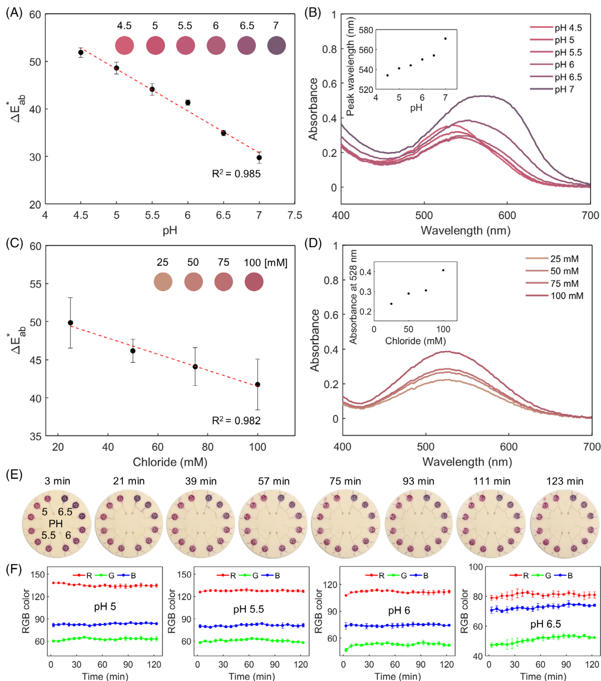
FIGURE 5 Quantitative colorimetric analysis of sweat pH and chloride concentration. (A–D) Standard calibration curves from an image processing algorithm and corresponding ultraviolet (UV)–visible spectroscopy results for various physiologically relevant levels of pH (A, B) and chloride concentration (C, D). The color intensity corresponds to the distance metric \Delta E_{ab}^* from the CIELAB color space, plotted as a function of chloride concentration and pH values. The color evolution in the standard calibration curves (A, C) and the presented color for each spectrum (B, D) correspond to the color exhibited at the detection reservoir in the device. The error bars in (A, C) represent one standard deviation of the three measurements of chloride concentrations or pH values corresponding to each standard level. (E, F) Colorimetric analysis of pH assay response as a function of time. Optical images of a device with 4 inlets (E) and extracted, averaged RGB color information at certain time points (F) during a 2-h period after the introduction of pH standard solutions with various pH values (5, 5.5, 6, and 6.5 for each group of reservoirs)
