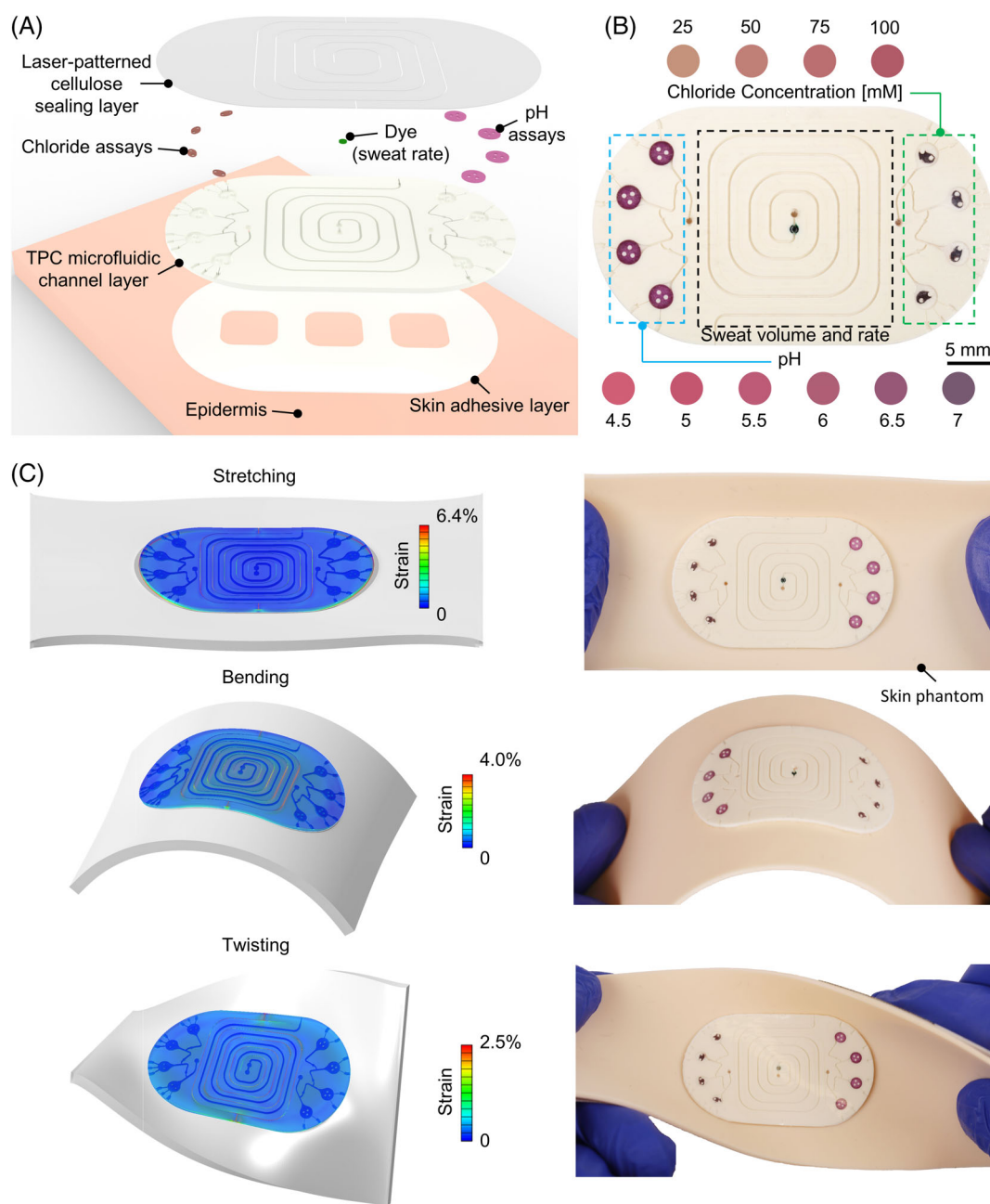
FIGURE 1 Soft, environmentally biodegradable microfluidic devices for sweat capture, storage and biomarker analysis. (A) Exploded view schematic illustration of the key layers and components of a representative device. TPC: thermoplastic copolyester elastomer. (B) Optical image of a device that includes a microfluidic channel for sweat volume and rate measurement, and reservoirs with colorimetric assays for pH and chloride analysis. The color evolution of both assays occurs over physiologically relevant ranges of chloride and pH in human sweat. (C) Finite element analysis results and respective optical images of the devices on silicone skin phantoms during stretching (25%), bending (radius of curvature 35 mm), and twisting (90°)
