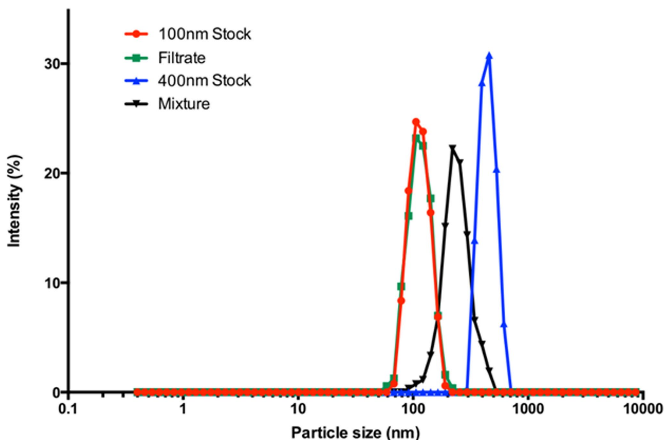
Fig. 7 Fractionation of 100 nm polystyrene NP from polydisperse mixture solution by using ultrasonic-assisted microfluidic particle sorting
