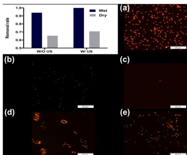
Fig. 6 Comparison of particle removal rate under different surface conditions (wet/dry). (a). 450 nm particles on a 400 nm filter after filtration. (b) and (c). Under wet conditions, most particles were removed with backflushing or ultrasonic cleaning, with no detectable particles remaining after ultrasonic treatment. (d) and (e). In dry conditions, significant fouling occurred
