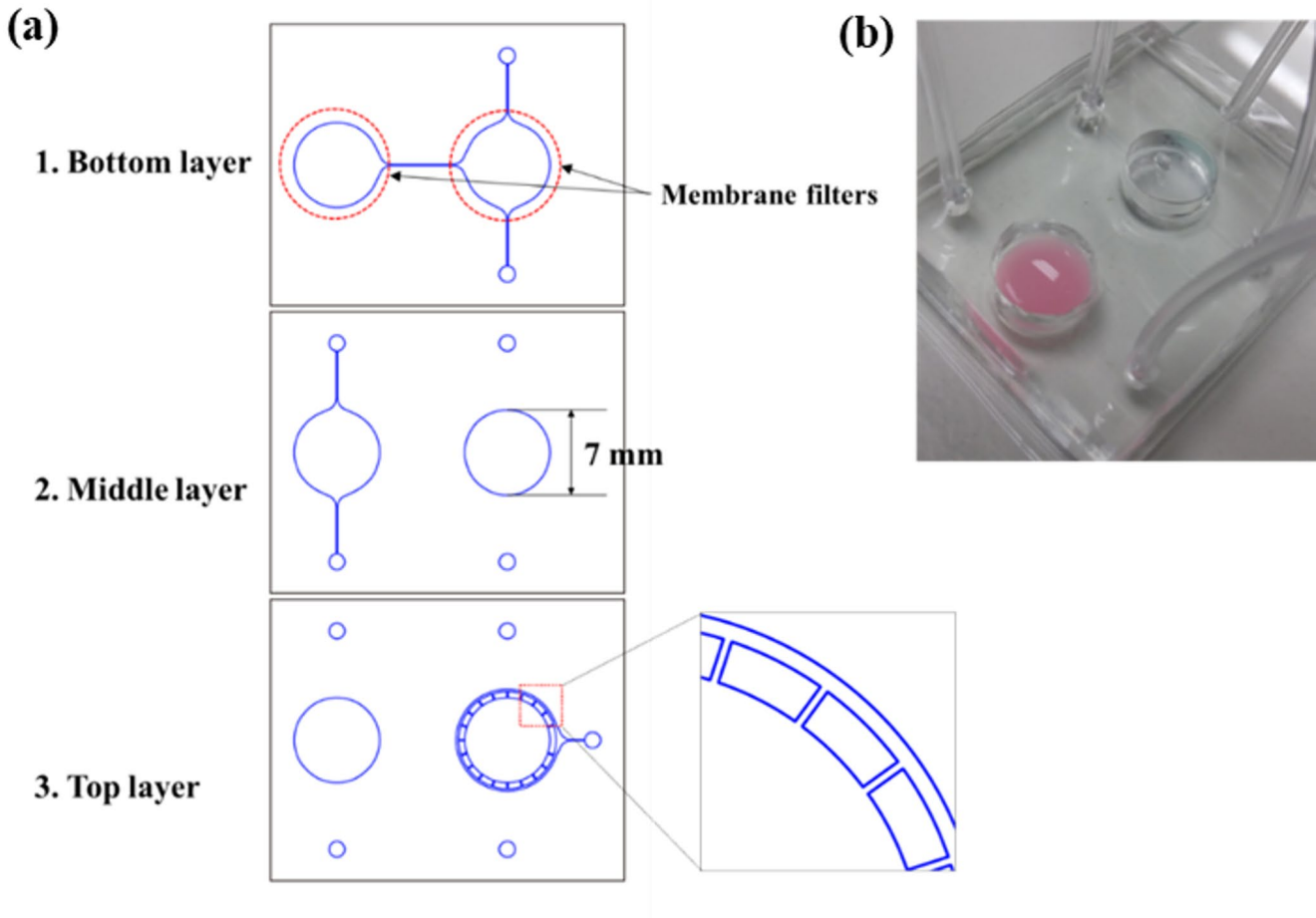
Fig. 3 Fabrication of microfluidic nanoparticle separation device. (a) Each PDMS layer was patterned by standard soft lithographic technique. Using an uncured PDMS prepolymer, membrane filters were embedded in the interface between the bottom and middle layers.
