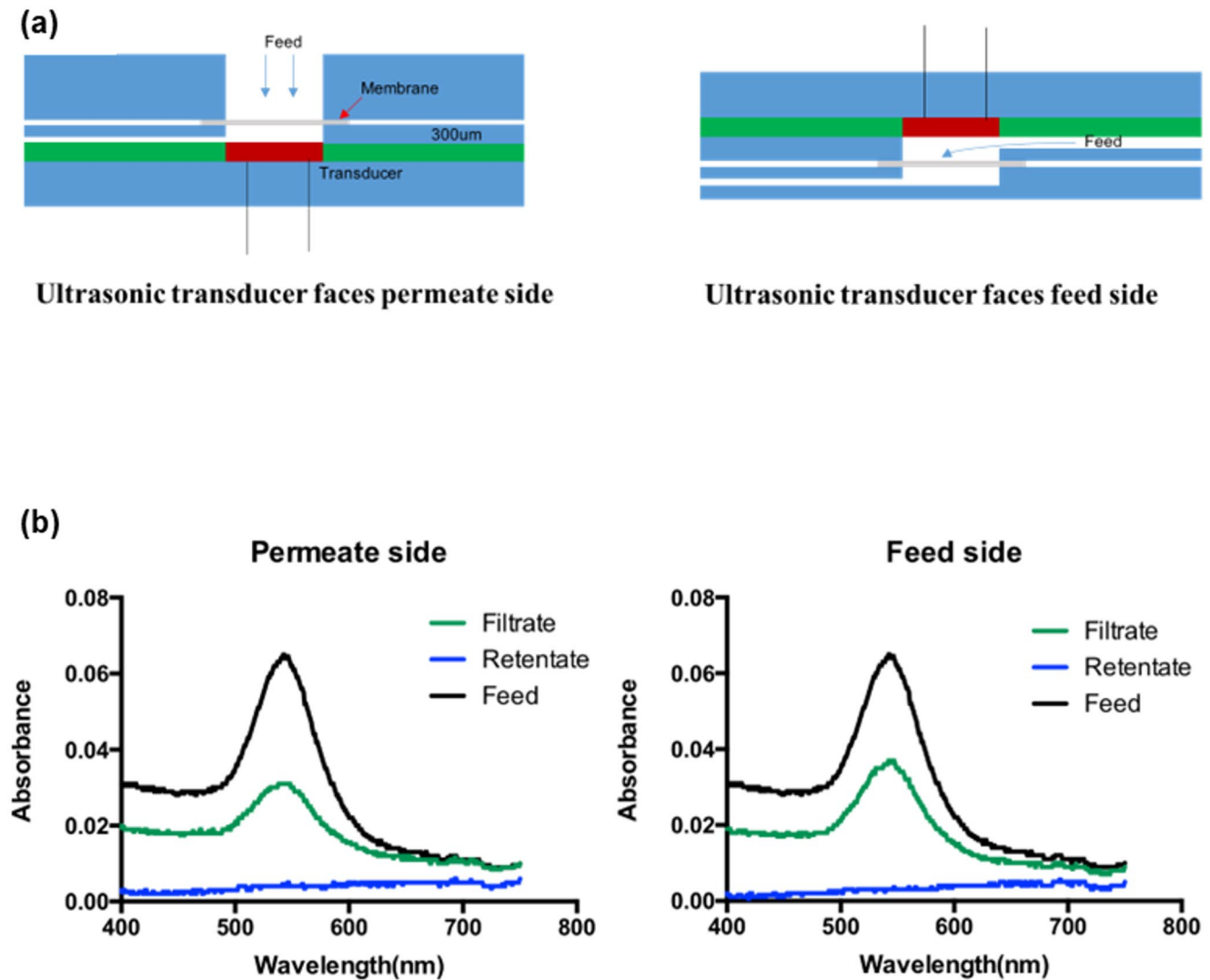
Fig. 8 Effect of the orientation of ultrasonic treatment on recovery rate. (a) Layouts of the microfluidic systems for particle filtration for ultrasonic treatment from the membrane filters' permeate side (left) and the feed side (right). The distance between the transducer and membrane remains 300 µm for the experiment. (b) Absorbance spectra of 60 nm
