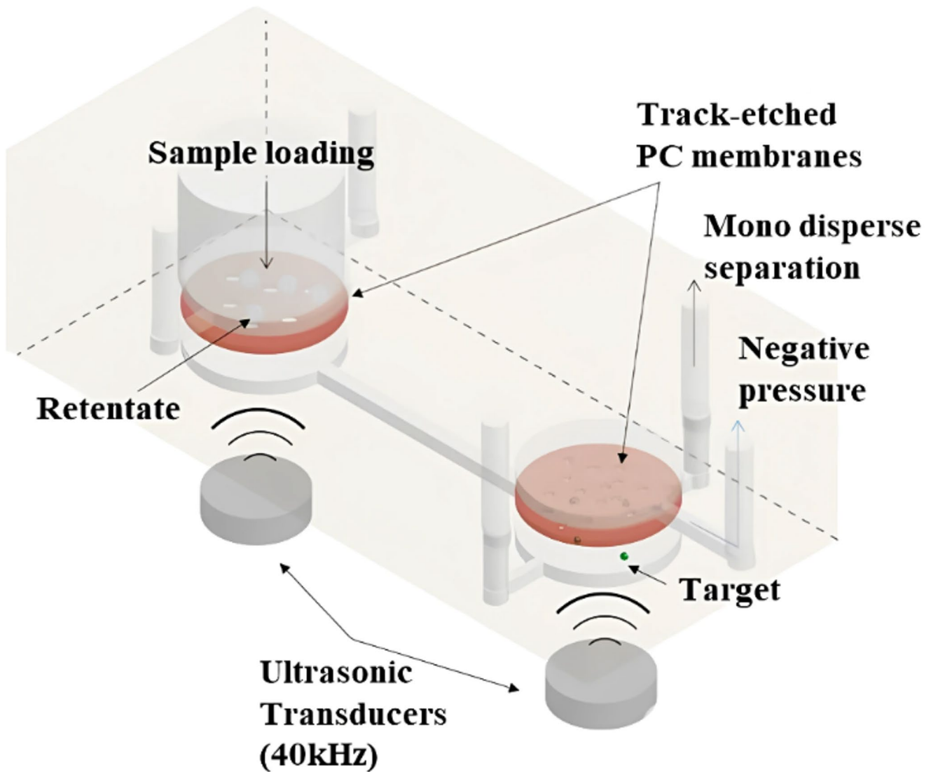
Fig. 1 Schematic of a microfluidic platform for nanoparticle separation
