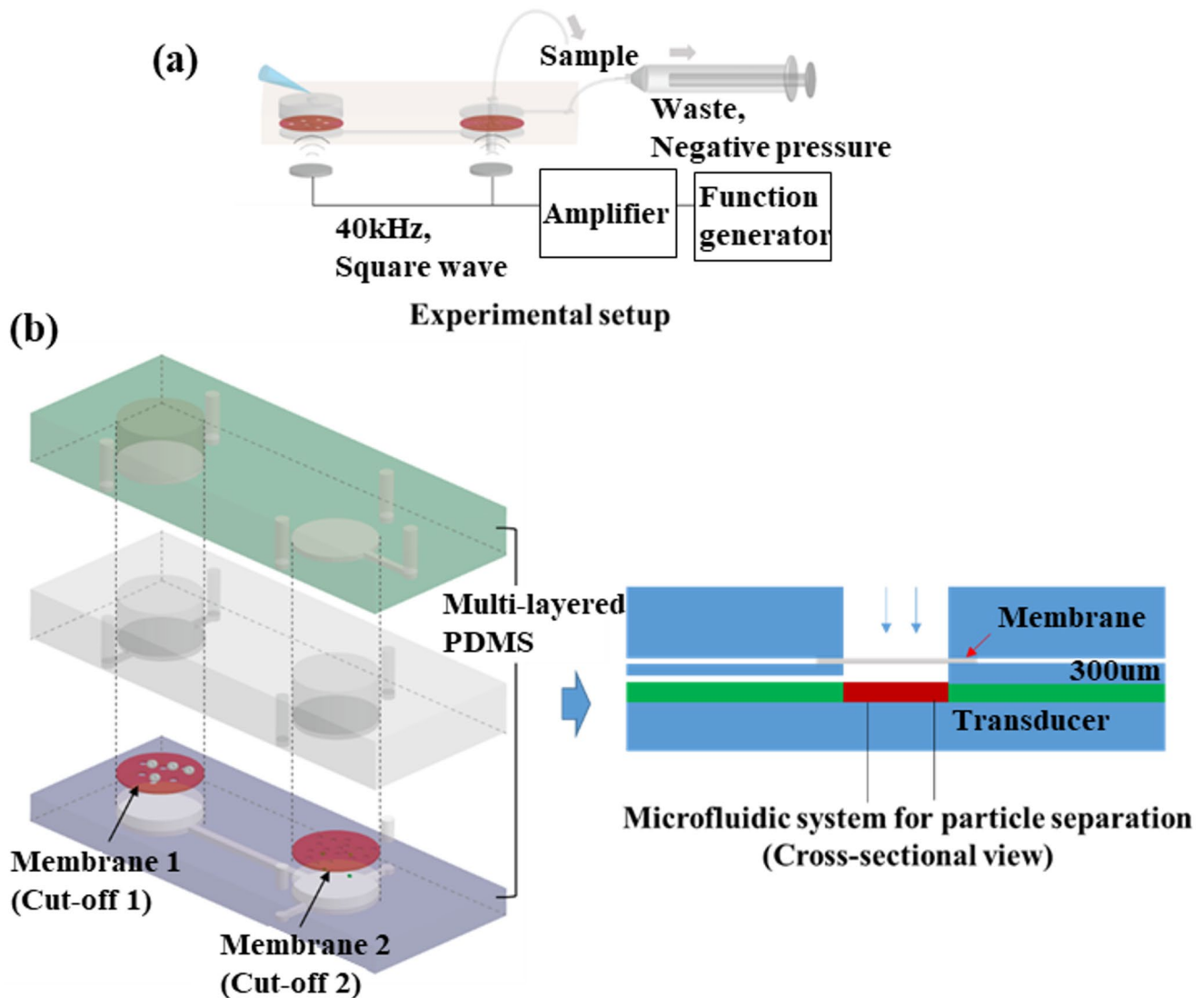
Fig. 4 Microfluidic device for on-chip nanoparticle separation consists of three PDMS layers. (a) Overall experimental setup (b) Membrane filters with different cut-off sizes (Cut-off 1 and Cut-off 2) were sandwiched between the bottom and middle layers for two different sizes nanoparticle separation. Particles larger than the cut-off of the first
