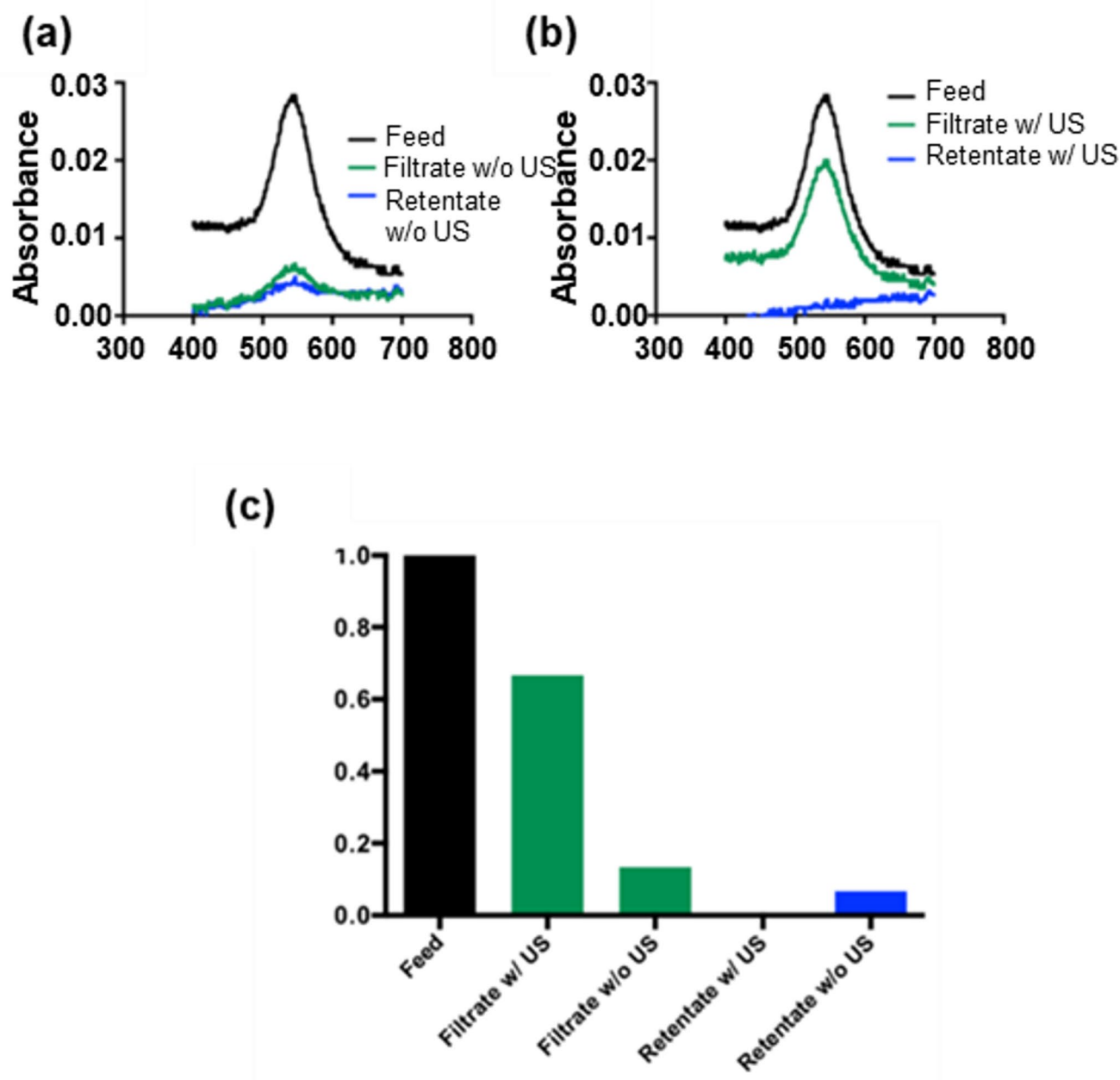
Fig. 5 60 nm Au NP filtration using membrane filter with 80 nm pore size cut-off embedded in the microfluidic size-based particle separation device. (a) The absorbance was measured using the feed, filtrate, and retentate sample collected after filtration without ultrasonic irradiation.
