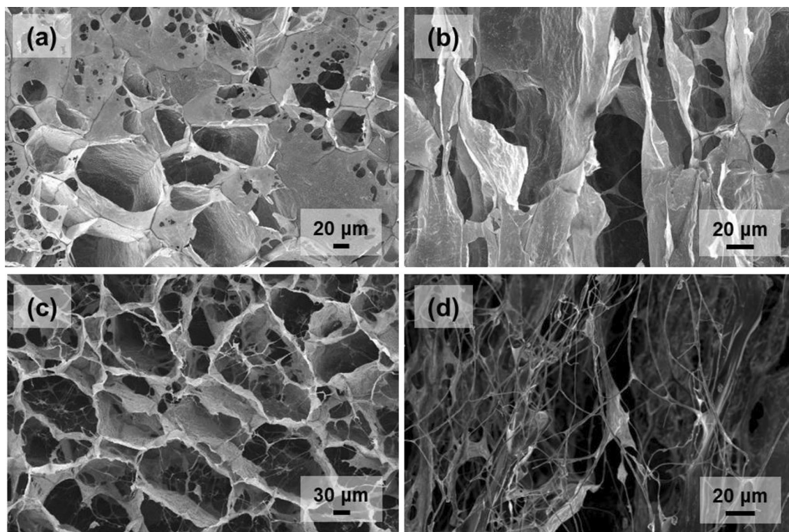
Fig. 2 SEM images of a the top view and b the side view for the normal CNF/AgNW-based aerogel. SEM images of c the top view and d the side view for the freeze-dried CNF/AgNW-based aerogel
