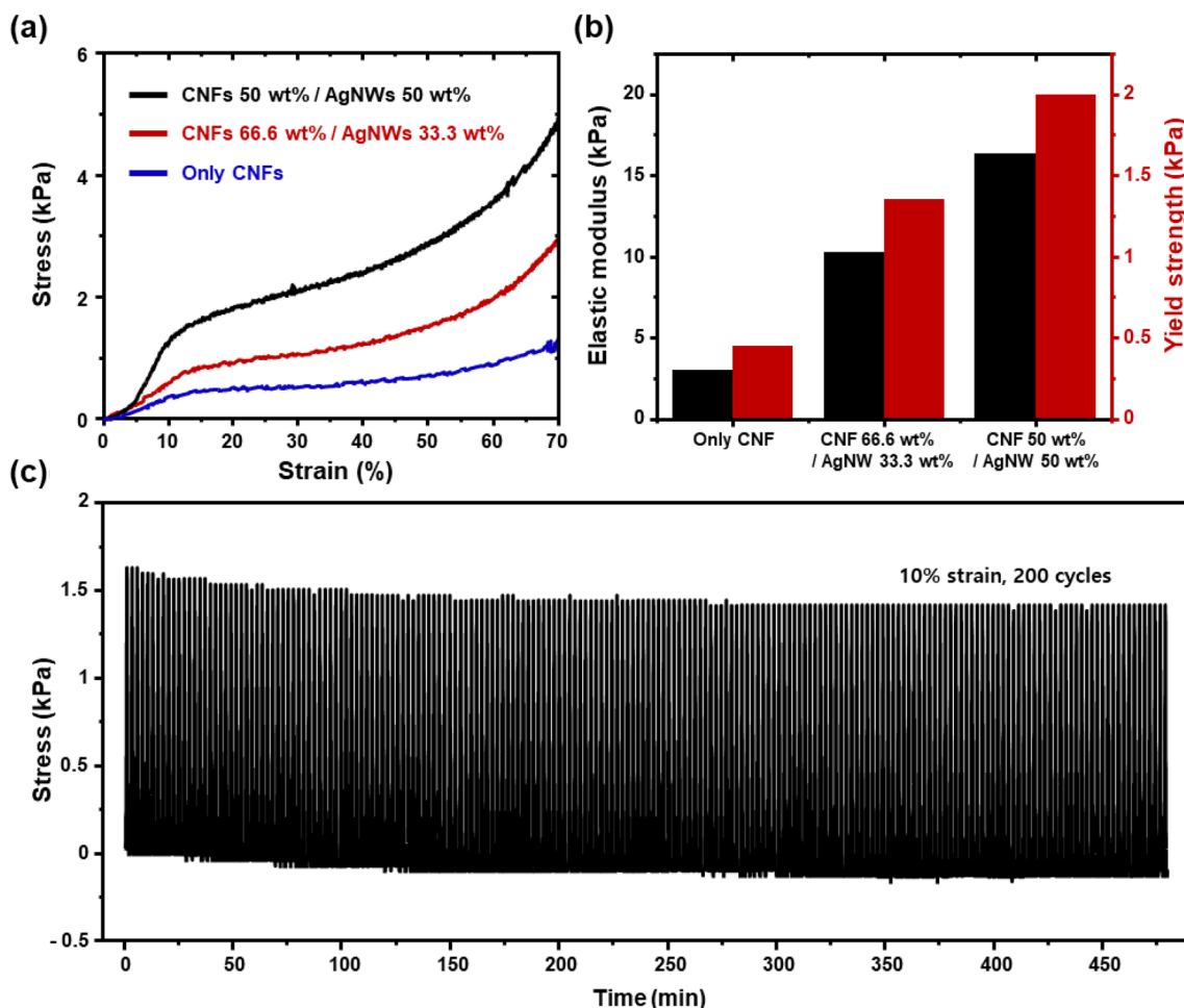
Fig. 3 Compressive mechanical properties of freeze-dried CNF-based aerogels. a Stress–strain curves of freeze-dried CNF-based aerogels with and without the addition of AgNWs. b Compressive elastic moduli and yield strengths of aerogels. Both mechanical properties are considerably increased when AgNW content increases. c Cyclic compressive test for 200 cycles of 10% strain for 50 wt% CNF/50 wt% AgNW aerogel
