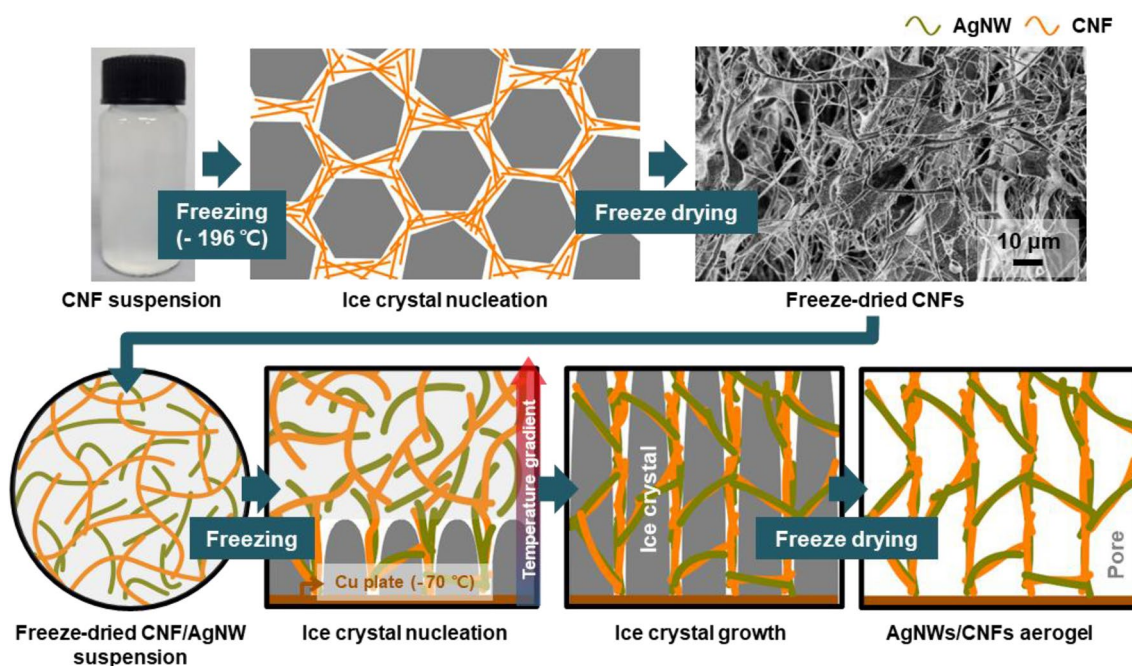
Fig. 1 Schematic of the fabrication process for the freeze-dried CNFs/AgNWs-based aerogel. The CNF suspension was directly frozen by LN 2 and freeze-dried. Then, the freeze-dried CNF/AgNW suspension was frozen, and ice crystals grew along the temperature gradient within the suspension. Once the freezing process was complete, the frozen suspension was subjected to freeze-drying. As a result, the freeze-dried CNFs/AgNWs-based aerogel with uniform distribution and assembly of microfiber-structured CNFs and AgNWs within the aerogel matrix is obtained
