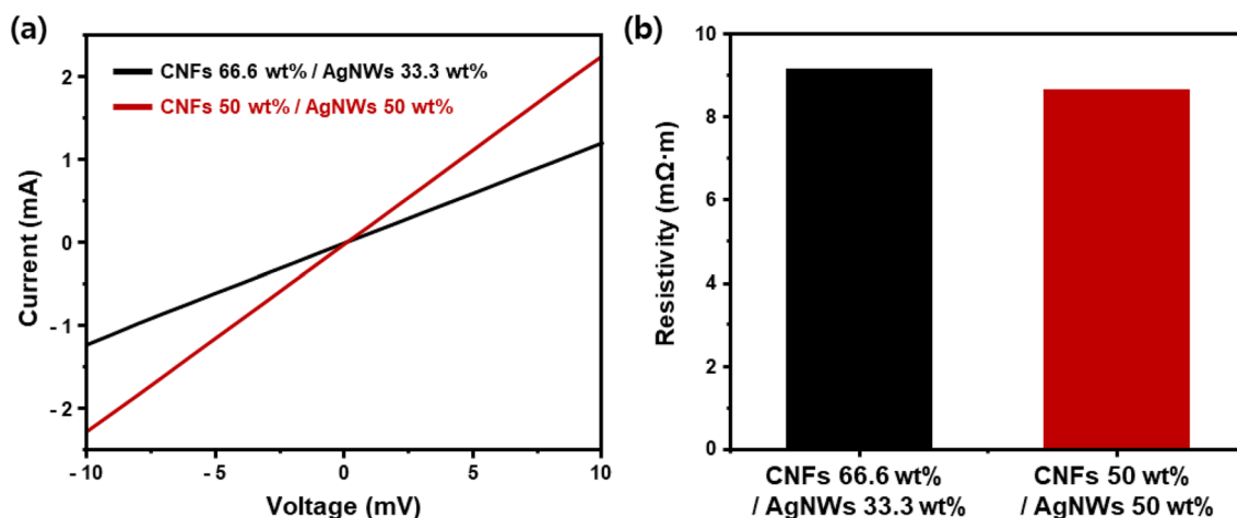
Fig. 4 Electrical properties of freeze-dried CNFs/AgNWs-based aerogels. a Linear I–V curves of metallic aerogels. b Electrical resistivity of aerogels with different compositions
