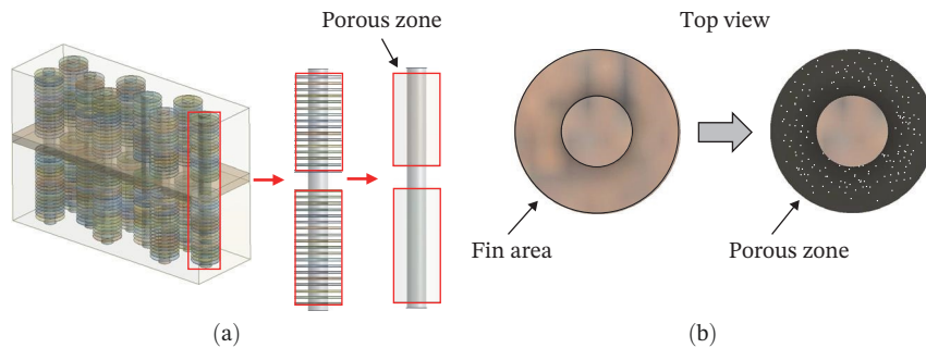
FIGURE 4 | Porous-medium representation of the finned tube. (a) Three-dimensional view of the finned tubes and corresponding porous regions. (b) Top view of the porous region. The porous-medium configuration reduces computational cost while preserving anisotropic flow resistance and heat transfer characteristics.
