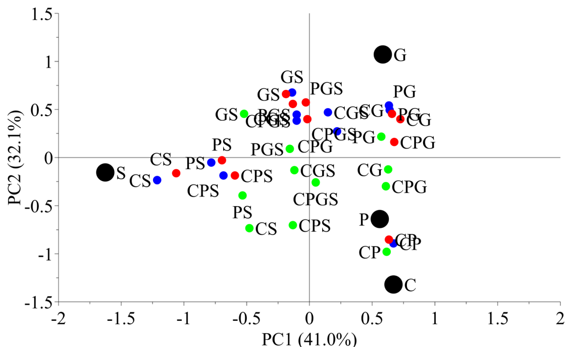
Fig. 12. PCA score plot based on ^1\text{H} NMR data of Coptis japonica (C), Phellodendron amurense (P), Gardenia jasminoides (G), Scutellaria baicalensis (S), and their mixtures. Black symbols represent single-herb extracts; blue symbols, co-extracted mixtures; red symbols, mixtures prepared by combining individually extracted components; and green symbols, computed average profiles calculated from the constituent single-herb spectra.
