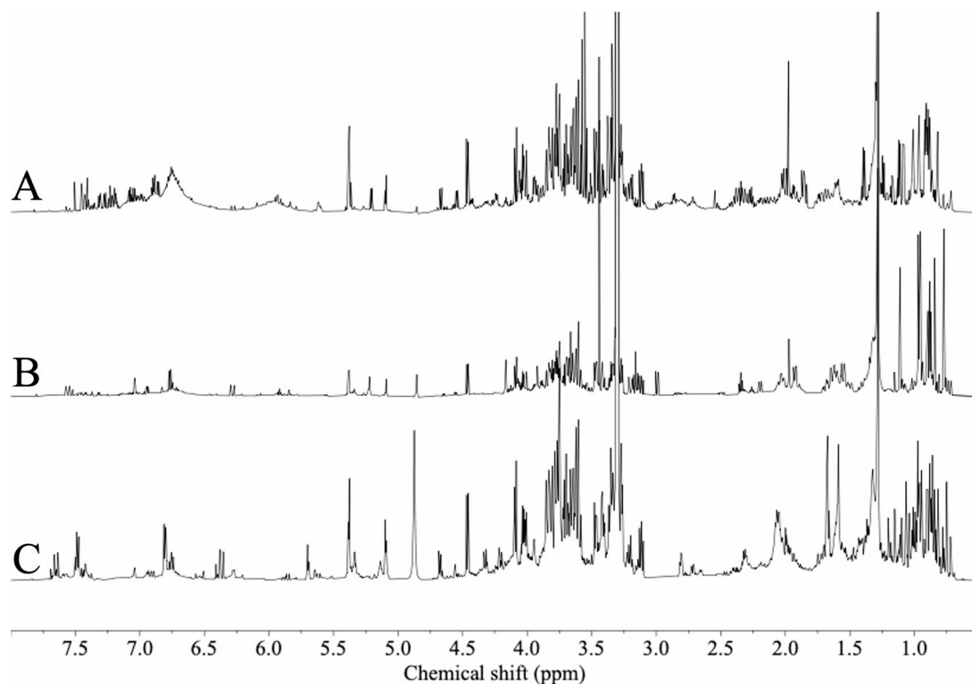
Fig. 7. Comparison of ^1\text{H} NMR spectra (600 MHz, \text{CH}_3\text{OH}-d_4 ) Uncaria tomentosa stem barks (NPL-NPL-018, A ), Uncaria rhynchophylla hooks (NPL-NPL-017, B ), and Vaccinium bracteatum stems (NPL-NET-001, C ).
