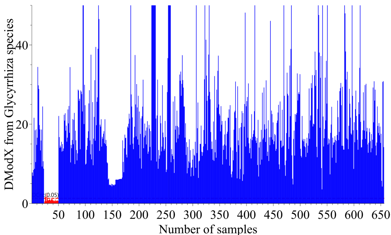
Fig. 3. Distance to the model (DModX) values from the cluster of Glycyrrhiza species to other samples. Glycyrrhiza species are in red marked by *. The SIMCA class model yielded R^2X(\text{cum}) = 0.933 and Q^2(\text{cum}) = 0.763 . Samples with DModX of each sample less than 1.0 are listed in (Table 3).
