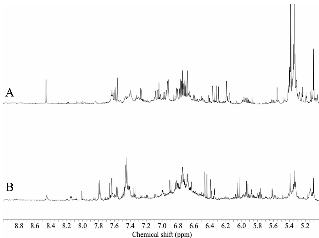
Fig. 6. Comparison of ^1\text{H} NMR spectra (600 MHz, \text{CH}_3\text{OH}-d_4 ) Taxus chinensis leaves (NPL-NPL-019, A ) and Viscum album stems (NPL-KIOM-020, B ).
