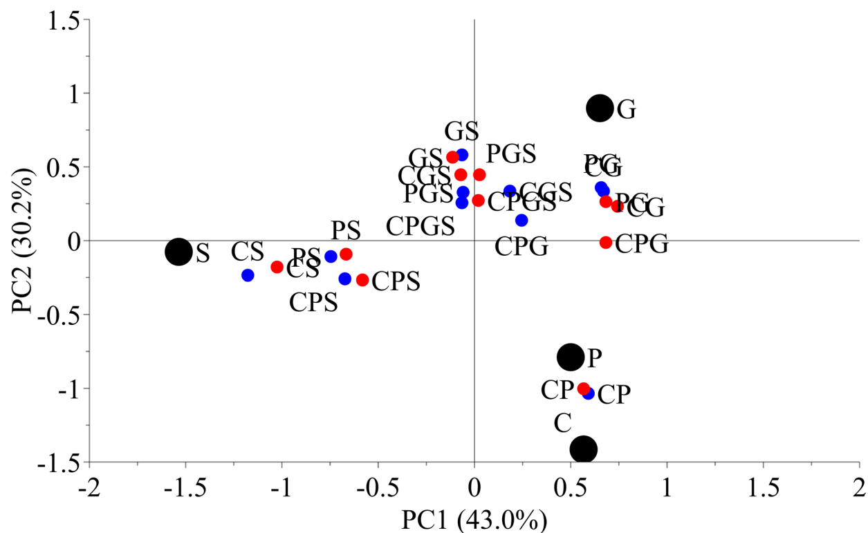
Fig. 10. Score plot of principal component analysis based on ^1\text{H} NMR data of Coptis japonica (C), Phellodendron amurense (P), Gardenia jasminoides (G), Scutellaria baicalensis (S), and their mixtures. Symbols in black are single plants, blue ones are co-extracted, and red ones are mixture of individually extracted ones.
