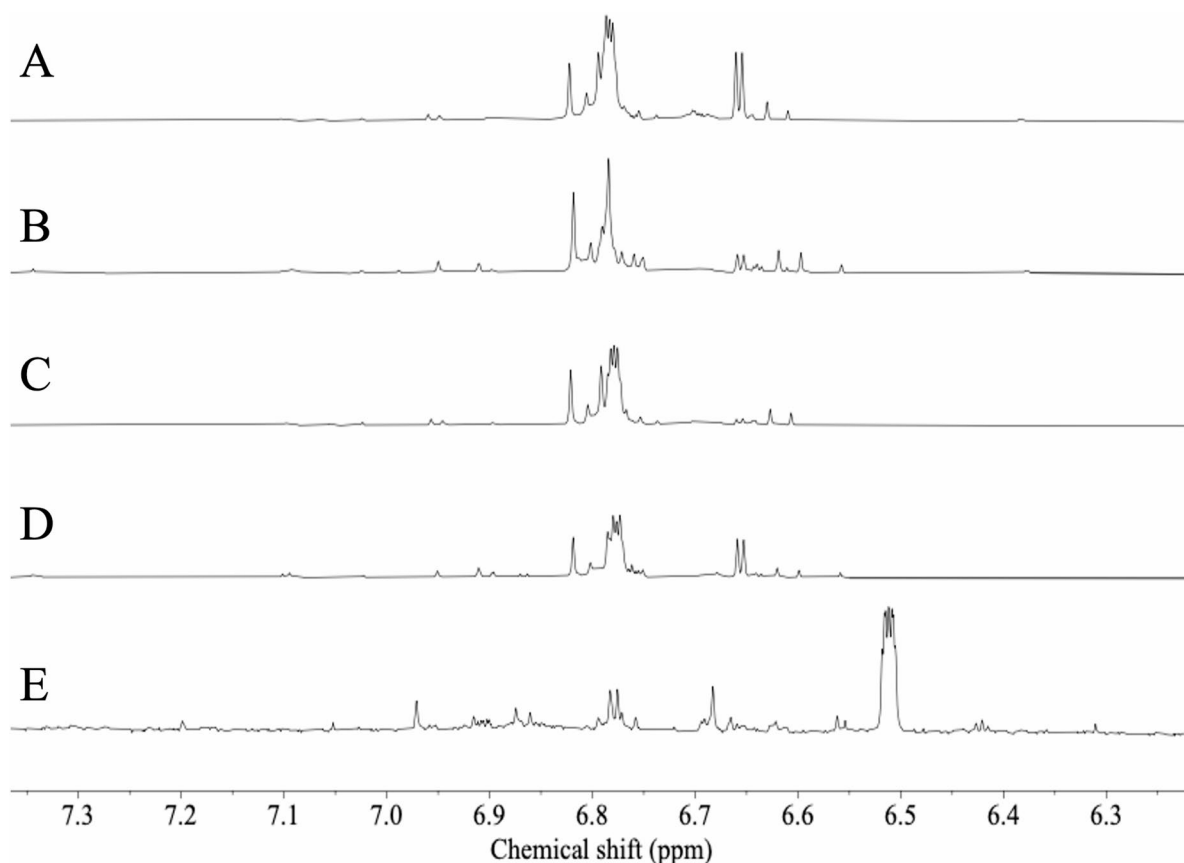
Fig. 5. ^1\text{H} NMR spectra (600 MHz, \text{CH}_3\text{OH}-d_4\text{-KH}_2\text{PO}_4 buffer (1:1, v/v, pH 6.0) of Schisandra chinensis fruits collected from Korea (A: NPL-KIOM-042, B: NPL-RDA-003, and C: NPL-NPL-045), from China (D: NPL-SUB-050), and from a market of the Netherlands (E).
