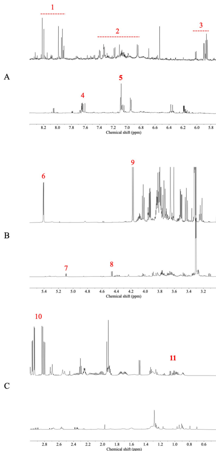
Fig. 1. ^1\text{H} NMR spectra of Astragalus membranaceus radix in the range of \delta 8.3–5.7 (A), \delta 5.6–3.0 (B), \delta 3.0–0.5 (C) measured in \text{CH}_3\text{OH}-d_4 - \text{KH}_2\text{PO}_4 buffer in \text{D}_2\text{O} (pH 6.0) (spectra on the top) and \text{CH}_3\text{OH}-d_4 (spectra on the bottom). 1: H-2 of isoflavonoids, 2: B-ring of flavonoids and isoflavonoids, 3: A-ring of flavonoids and isoflavonoids, 4: H-2' and H-6' of kaempferol analogues, 5: H-3' and H-5' of kaempferol analogues, 6: H-1 of sucrose, 7: H-1 of \alpha -glucose, 8: H-1 of \beta -glucose, 9: H-2' of sucrose, 10: aspartic acid and asparagine, 11: methyls of saponins.
