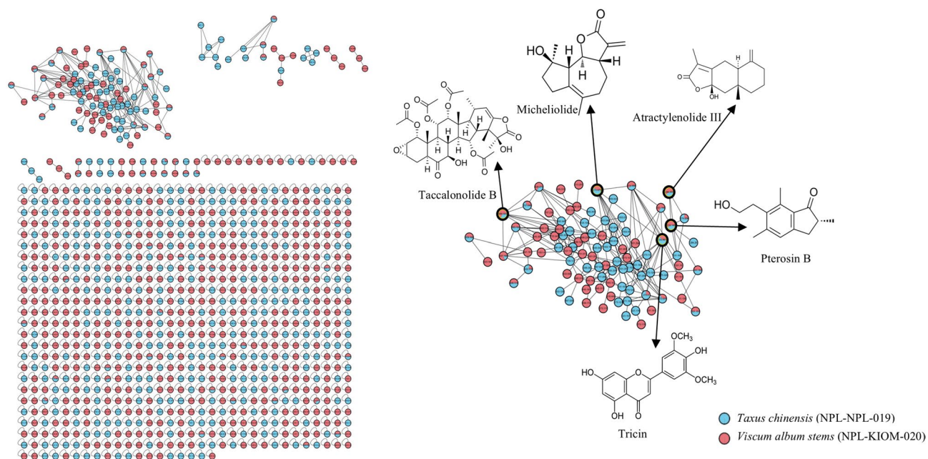
Fig. 8. Feature-based molecular networking (FBMN) of taxonomically distinct medicinal plants highlighting metabolite overlaps and functional similarity. The network generated from UHPLC-DAD-QToF-MS data of the Taxus chinensis and Viscum album using ion identity molecular networking (IIMN) shows shared molecular families, including a lactone-related cluster, observed across both species. Node labels correspond to feature IDs, and the corresponding precursor m/z , RT, library match information, and MSI confidence levels are provided in Supplementary Table S2.
