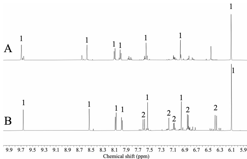
Fig. 11. Comparison between ^1\text{H} NMR spectra of Coptis japonica (A) and Phellodendron amurense (B). 1: ^1\text{H} resonances of berberine. 2: ^1\text{H} resonances of chlorogenic acid.
