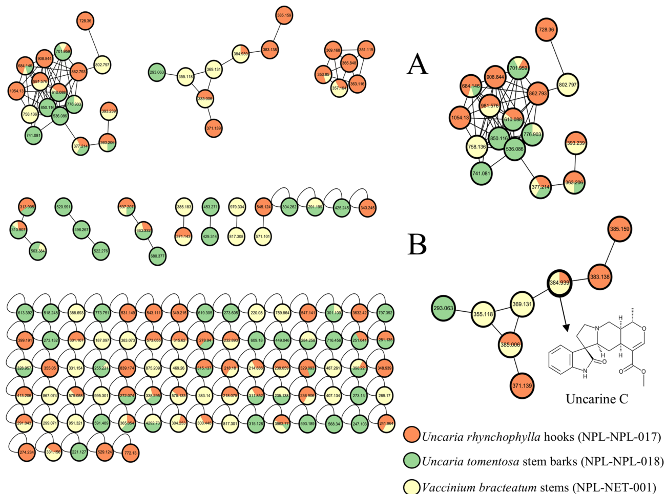
Fig. 9. Comparative FBMN analysis of Uncaria tomentosa , Uncaria rhynchophylla , and Vaccinium bracteatum , highlighting shared alkaloid and polyphenol clusters. (A) Molecular networking revealed clusters in alkaloid and polyphenol features. (B) Enlarged view of a representative cluster showing features putatively annotated as uncarine C and structurally related polyphenolic glycosides detected across all three species. Highlighted nodes are traceable to their feature IDs and corresponding annotation details, including precursor m/z , RT, library match information, and MSI confidence levels, provided in Supplementary Table S3.
