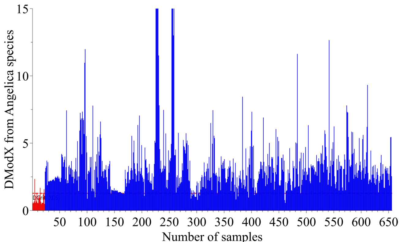
Fig. 2. Distance to the model (DModX) values from the cluster of Angelica species to other samples. Angelica species are in red marked by *. The SIMCA class model yielded R^2X(\text{cum}) = 0.691 and Q^2(\text{cum}) = 0.549 . Samples with DModX of each sample less than 1.0 are listed in (Table 2).
