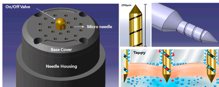
Figure 1. Schematic diagram of the microneedle device (Tappy Tok Tok ® ). (Reproduced from Eum et al. J Biomed Eng Res 2012; 33; 202–206, with permission of The Korean Society of Medical and Biological Engineering [11].).
