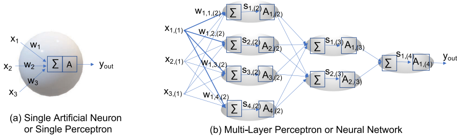
Fig. 2. Perceptron and neural network model.
