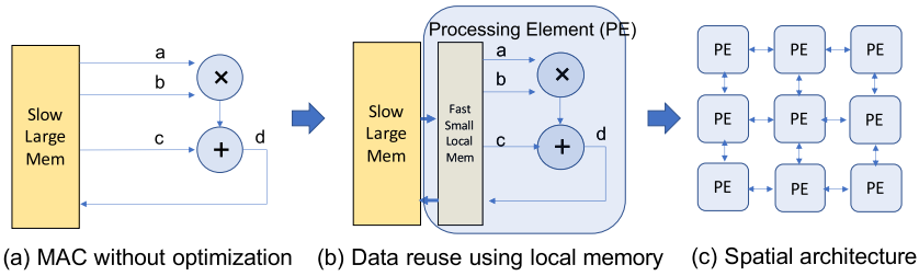
Fig. 9. MAC dataflow.
