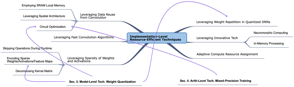
Fig. 8. Categorization of implementation-level resource-efficient techniques.
