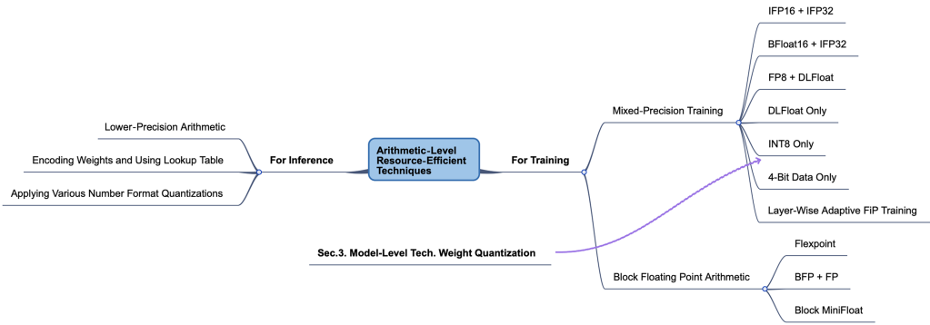
Fig. 7. Categorization of arithmetic-level resource-efficient techniques.
