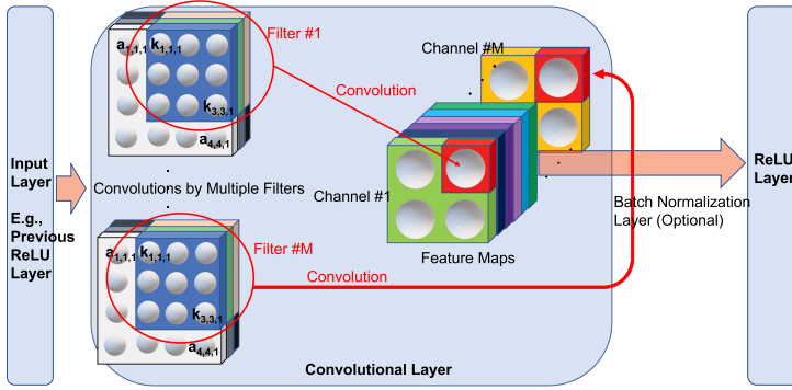
Fig. 3. Convolution operations in a CNN.
