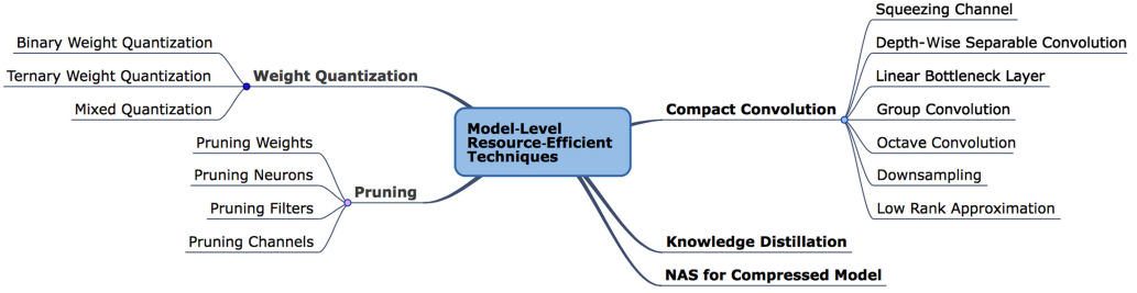
Fig. 4. Categorization of model-level resource-efficient techniques.
