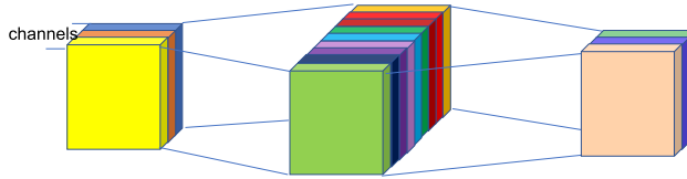
Fig. 6. Bottleneck layer block used in the work of Sandler et al. [142].
