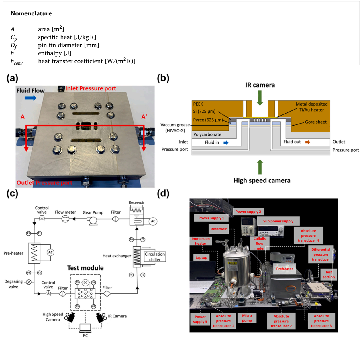
Fig. 1. Experimental setup and test section. (a) Photograph of the assembled test module, (b) Cross-sectional side view of the test module, (c) Schematic configuration of the flow loop, and (d) Photo of the equipment in the flow loop.
