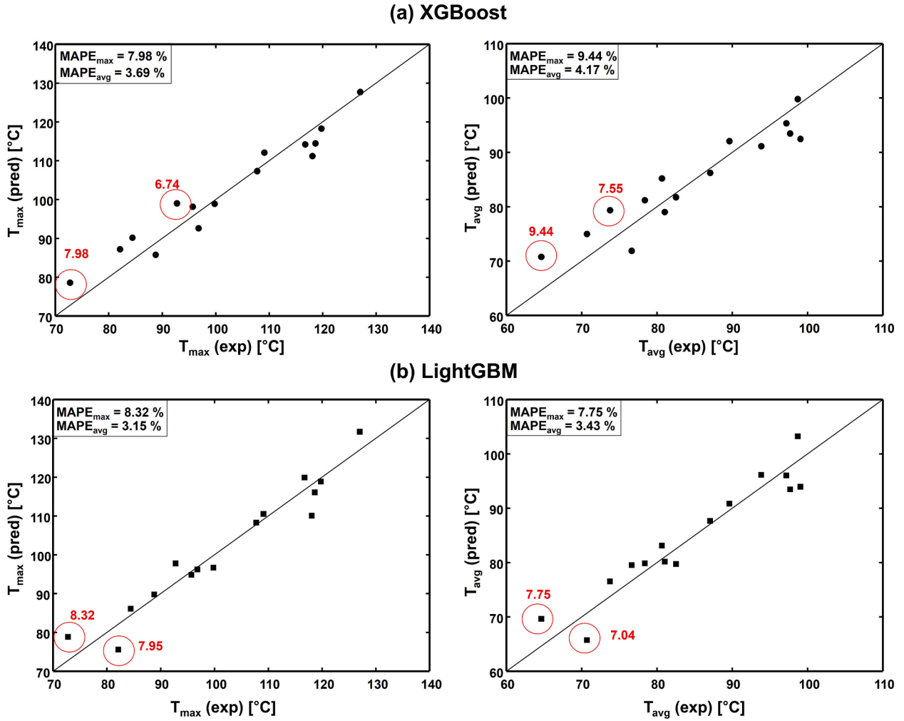
Fig. 7. Comparison of experimental and predicted scalar-form heated surface temperature. Predictive results using two specific ML algorithms: (a) XGBoost, (b) LightGBM.
