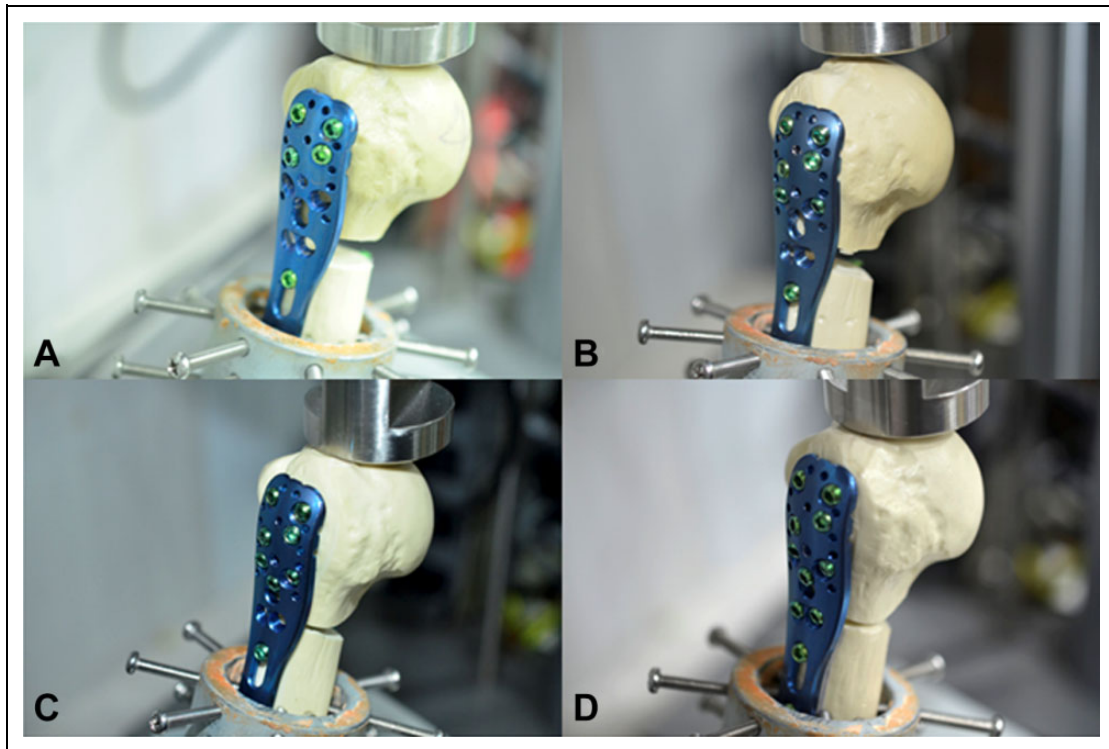
Figure 3. Four groups of fixation model. (A) 4-screw group, (B) 6-screw group, (C) 7-screw group, and (D) 9-screw group.
