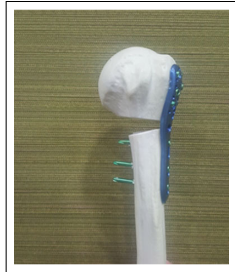
Figure 1. Preparation of the fracture model. Medially based wedge osteotomy was made 1 cm inferior to the articular margin to simulate surgical neck fractures with significant comminution.
