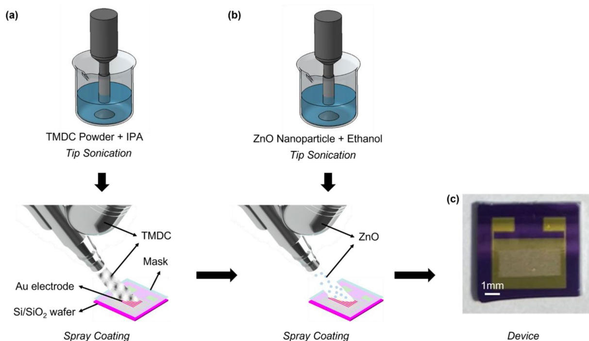
Fig. 1 Schematic of TMDC/ZnO-based \text{NO}_2 gas sensor fabrication process. (TMDC: transition metal dichalcogenides; IPA: Isopropylalcohol)
