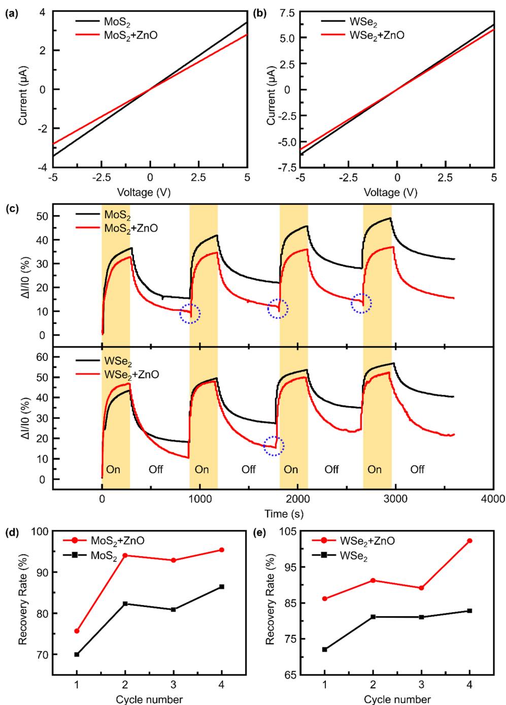
Fig. 4 I-V characteristics of a MoS 2 , MoS 2 /ZnO, b WSe 2 and WSe 2 /ZnO-based gas sensor in air environment at 100 °C. c Gas sensing response of transition metal dichalcogenides (TMDC)-based gas sensor to 10 ppm NO 2 gas at 100 °C. The part where the conductivity decreased at the early stage of NO 2 exposure is outlined by the blue dotted line. d Recovery rate per cycle of MoS 2 and MoS 2 /ZnO-based gas sensor. e Recovery rate per cycle of WSe 2 and WSe 2 /ZnO-based gas sensor
