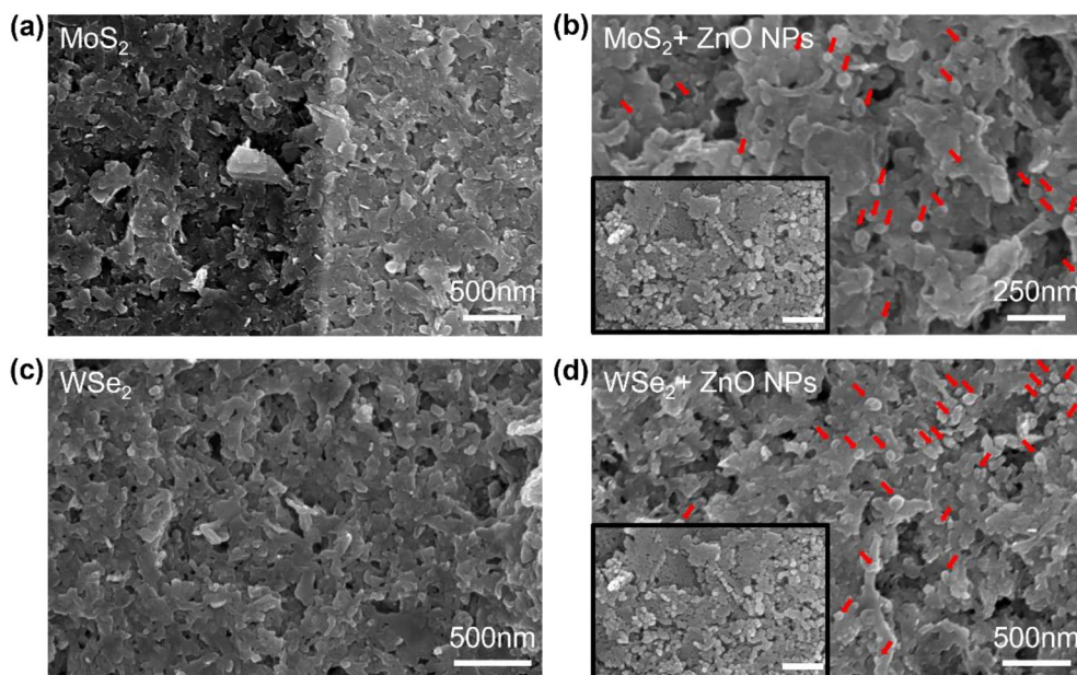
Fig. 2 Scanning electron microscopic images of a MoS 2 , b MoS 2 /ZnO-, c WSe 2 -, d WSe 2 /ZnO-based gas sensors. The red arrow represents the ZnO nanoparticles (NP). The insets in b and d show SEM image of undiluted ZnO nanoparticles. The scale bars in the insets are 250 nm
