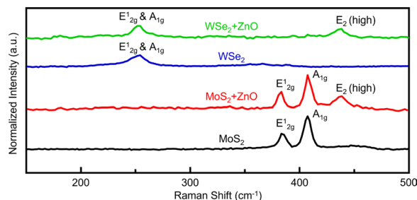
Fig. 3 Raman spectra of the transition metal dichalcogenides (TMDC)-based gas sensor (excited by 532 nm laser). Unlike TMDC, the TMDC/ZnO sensor exhibits the E 2 (high) characteristic peak of ZnO
