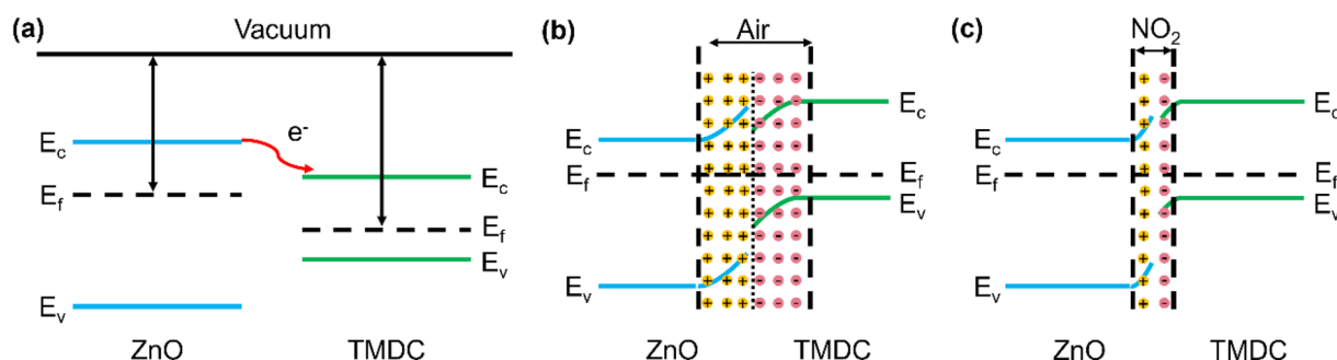
Fig. 5 Band diagrams of transition metal dichalcogenides (TMDC)/ZnO heterojunction a before equilibrium, b after equilibrium in air and c \text{NO}_2 gas atmosphere
