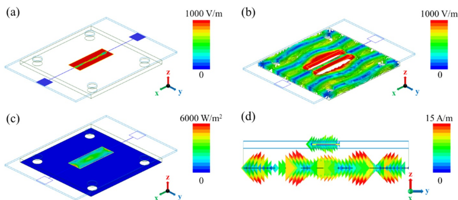
FIGURE 3 | (a) Electric-field distribution on the ITO layer and bias line. (b) Electric-field distribution within the substrate. (c) Surface loss density. (d) Surface current density.
