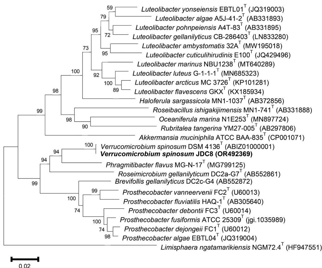
Fig. 4. Neighbor-joining phylogenetic tree based on 16S rRNA gene sequences showing the relationship between the strains isolated in this study and their relatives in the family Verrucomicrobiaceae of the phylum Verrucomicrobiota. Bootstrap values (> 50%) are shown at branching points. Limisphaera ngatamarikiensis NGM72.4 T used as an outgroup. Scale bar, 0.02 substitutions per nucleotide.
