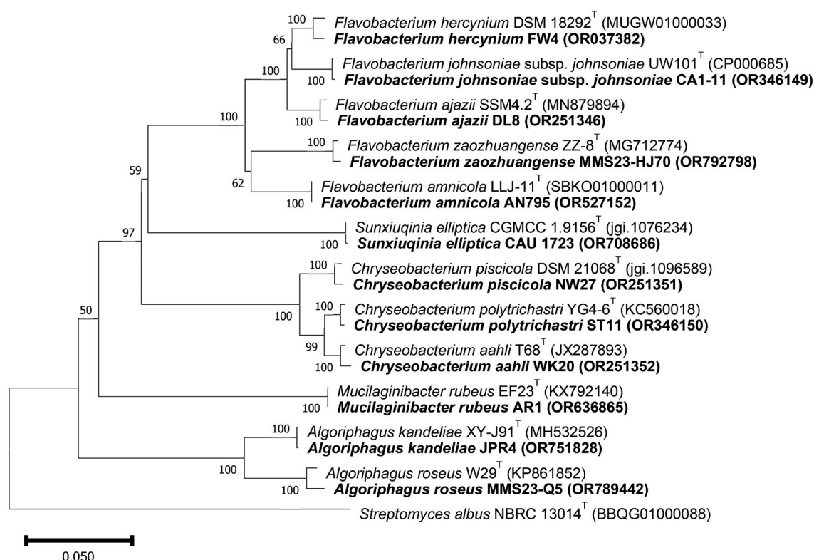
Fig. 3. Neighbor-joining phylogenetic tree based on 16S rRNA gene sequences showing the relationship between the strains isolated in this study and their relatives in the families Cyclobacteriaceae , Flavobacteriaceae , Prolixibacteraceae , Sphingobacteriaceae and Weeksellaceae of the phylum Bacteroidota . Bootstrap values (>50%) are shown at branching points. Streptomyces albus NBRC 13014 T used as an outgroup. Scale bar, 0.05 substitutions per nucleotide.
