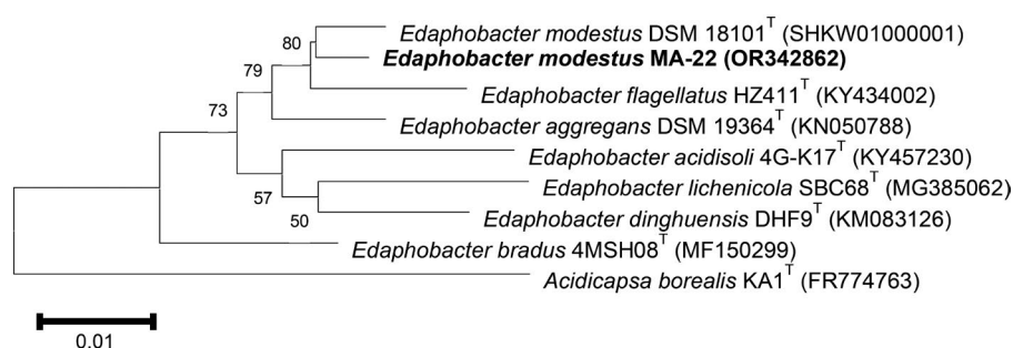
Fig. 2. Neighbor-joining phylogenetic tree based on 16S rRNA gene sequences showing the relationship between the strains isolated in this study and their relatives in the family Acidobacteriaceae of the phylum Acidobacteriota . Bootstrap values (>50%) are shown at branching points. Acidicapsa borealis KA1 T used as an outgroup. Scale bar, 0.01 substitutions per nucleotide.
