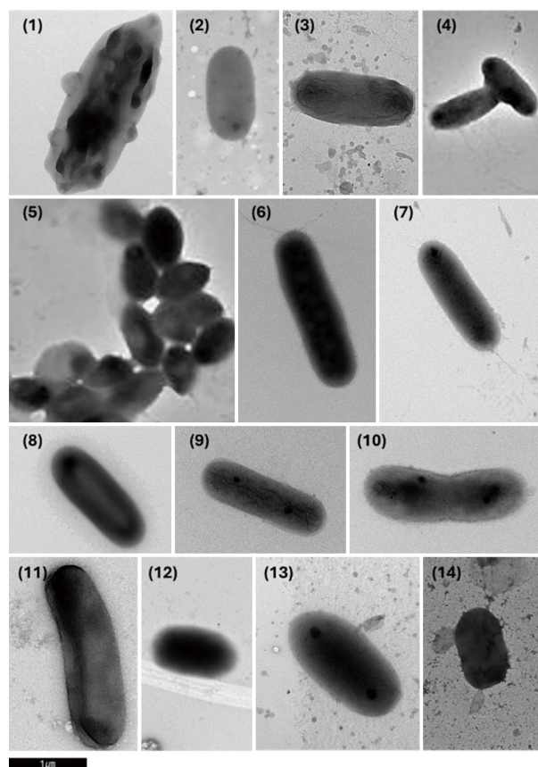
Fig. 1. Transmission electron or scanning electron micrographs of cells of the strains isolated in the study. Strain: 1, MA-22; 2, MMS23-Q5; 3, JPR4; 4, AN795; 5, CA1-11; 6, DL8; 7, FW4; 8, MMS23-HJ70; 9, CAU 1723; 10, AR1; 11, ST11; 12, WK20; 13, NW27; 14, JDC8. Scale bar, 1 \mu m.
