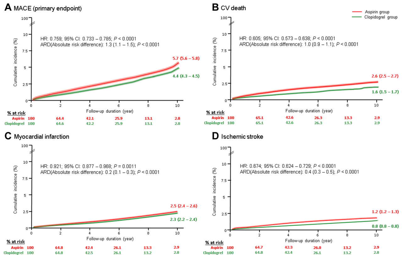
FIGURE 2 Cumulative Risk of Effectiveness Outcomes After IPTW
