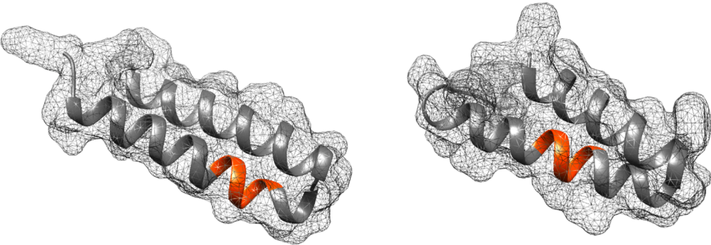
Fig. 3. Structural conformation of salivaricin P chain \alpha (left) and chain \beta (right). The highlighted orange regions represent the GXXXG motif.
