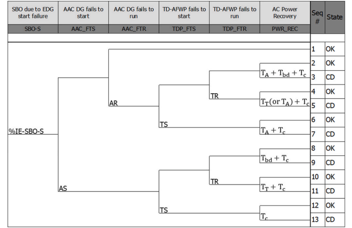
Fig. 2. Proposed consideration of AAC DG and TDP failures in the convolution approach.
