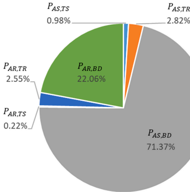
Fig. 5. SBO CCDP contribution of sequence probabilities (calculated with the convolution approach).
